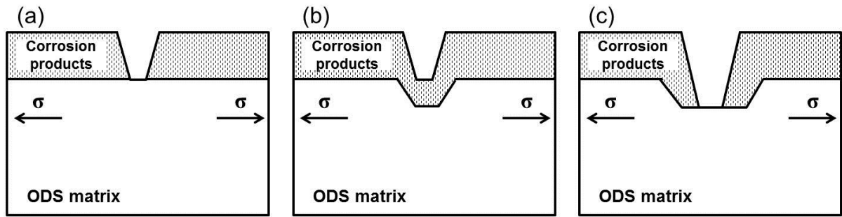
Fig. 3.10. Schematic view of “corrosion layer cracking” model of ODS steel in SCPW.
