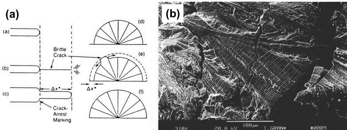
Fig. 4.22 (a) schematic drawing of the transgranular SCC process and the mechanism of striation formation. (After Refs. 29–33. Courtesy of NACE.) (b) Crack arrest marks on a transgranular SCC surface, observed near the overload region on a slow strain rate specimen ( 10^{-5} \text{ s}^{-1} ) of 70–30 brass tested in pH 7.2 Mattsson's [35] solution with 0.05M NaCl
