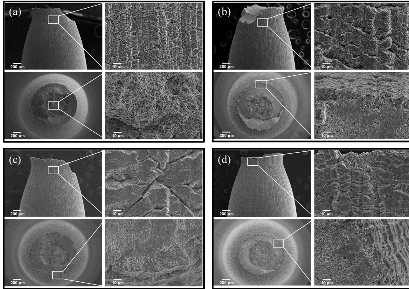
Fig. 3.5. SEM images of fracture surface and gauge section of the ODS steel after SSRT at lower strain rate of 1 \times 10^{-6} \text{ s}^{-1} or 5 \times 10^{-7} \text{ s}^{-1} . (a : vacuum - 1 \times 10^{-6} \text{ s}^{-1} , b : SCPW with DH 0.4 ppm - 1 \times 10^{-6} \text{ s}^{-1} , c : SCPW with DO & DH < 0.01 ppm - 1 \times 10^{-6} \text{ s}^{-1} , d : SCPW with DO 8.0 ppm - 5 \times 10^{-7} \text{ s}^{-1} )
