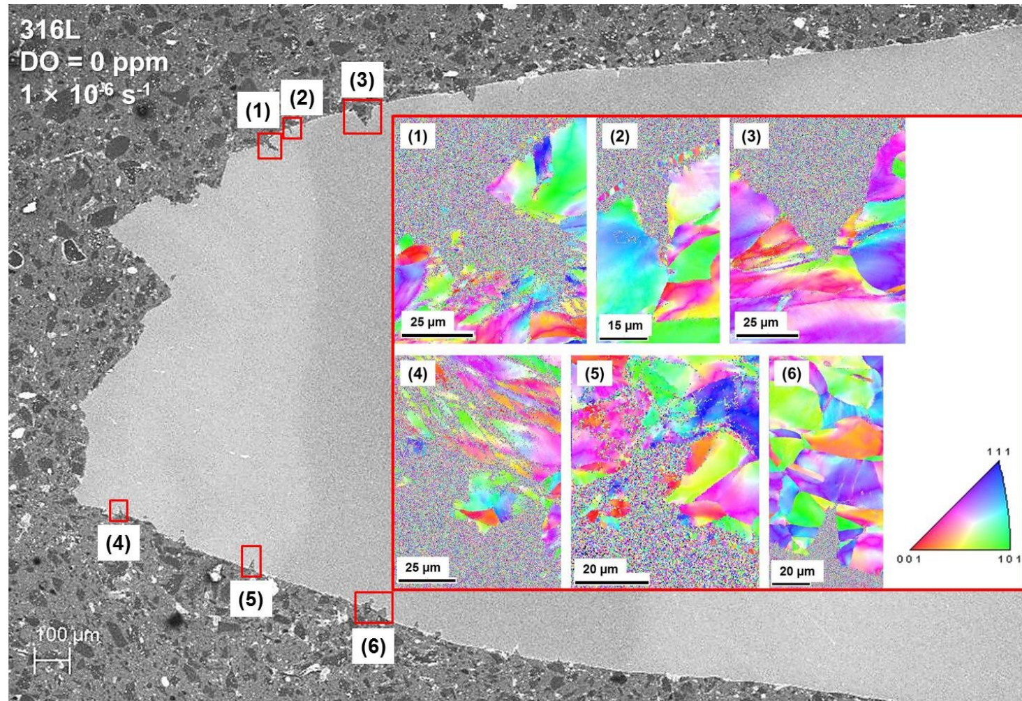
Fig. 4.16 EBSD analysis results of cracks on SUS316L after SSRT at lower strain rate of 1 \times 10^{-6} \text{ s}^{-1} in deaerated SCPW (DO & DH < 0.01 ppm)
