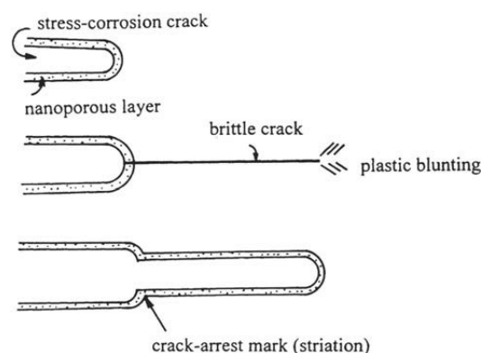
Fig. 4.21 Schematic drawing of crack growth by film-induced cleavage in an fcc metal or alloy. [34]
