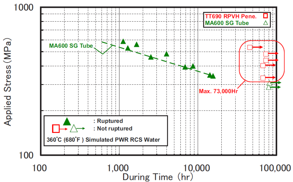
Fig. 2.17. Results of PWSCC tests on alloy 690 base metal and Alloy 600 base metal showing no cracking detected in alloy 690 after test times up to ~75 000 hours.
