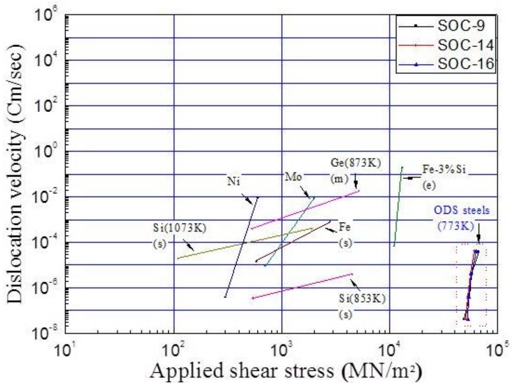
Fig. 6.3. The dependence of dislocation velocity on applied shear stress with various kinds of materials and ODS steels
