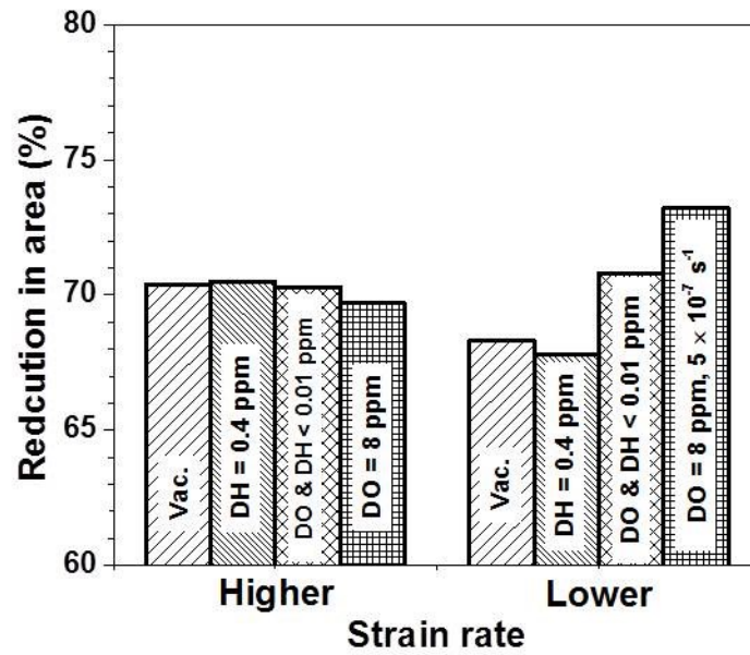
Fig. 3.3. Reduction in area of ODS ferritic steel after SSRT at higher ( 1 \times 10^{-3} \text{ s}^{-1} ) and lower ( 1 \times 10^{-6} \text{ s}^{-1} or 5 \times 10^{-7} \text{ s}^{-1} ) strain rates.
