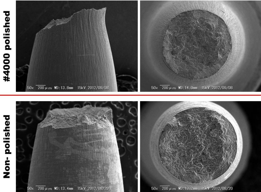
Fig. 5.8. Fracture surface and gauge section of the round bar specimen with different surface condition after SSRT in SCPW at lower strain rate ( 1 \times 10^{-6} \text{ s}^{-1} )
