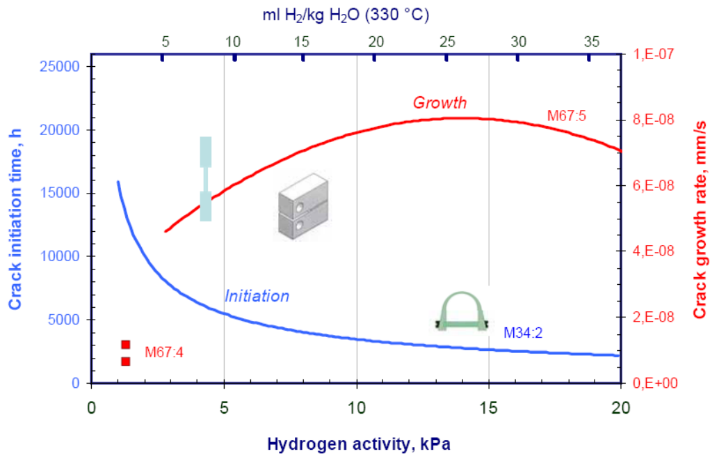
Fig. 2.14. Comparison of the effect of hydrogen on initiation and propagation of PWSCC in alloy 600 MA [7].
