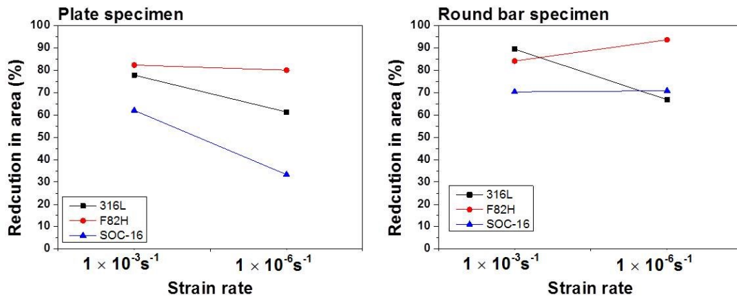
Fig. 5.5 Reduction in area as a function of strain rate with different specimen shapes.
