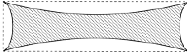
Fig. 5.7. Sketch of end view of rectangular test piece after fracture showing constraint at corners indicating the difficulty of determining reduced area.
