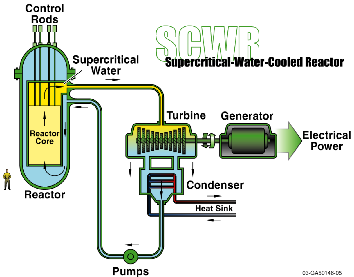
Fig. 2.8: The outline of a supercritical water cooled power plant. The power plant utilizes a direct steam cycle and, thanks to the properties of supercritical water, requires no steam driers or recirculation usually encountered in NPPs [26].
