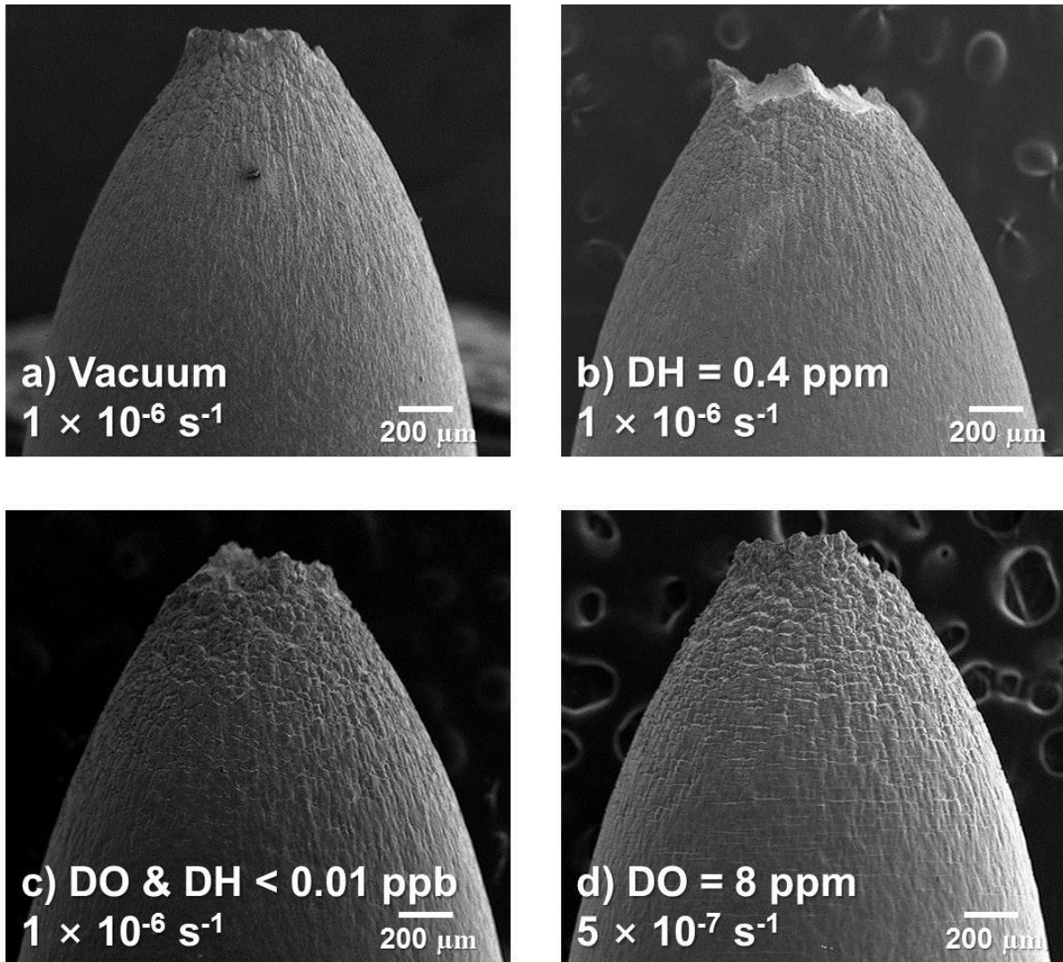
Fig. 4.11 Specimen side surface of F82H ferritic / martensitic steel after SSRT at lower strain rate of 1 \times 10^{-6} \text{ s}^{-1} or 5 \times 10^{-7} \text{ s}^{-1} in a) vacuum, b) SCPW with DH 0.4 ppm, c) deaerated SCPW (DO & DH < 0.01 ppb) and d) SCPW with DO 8 ppm.
