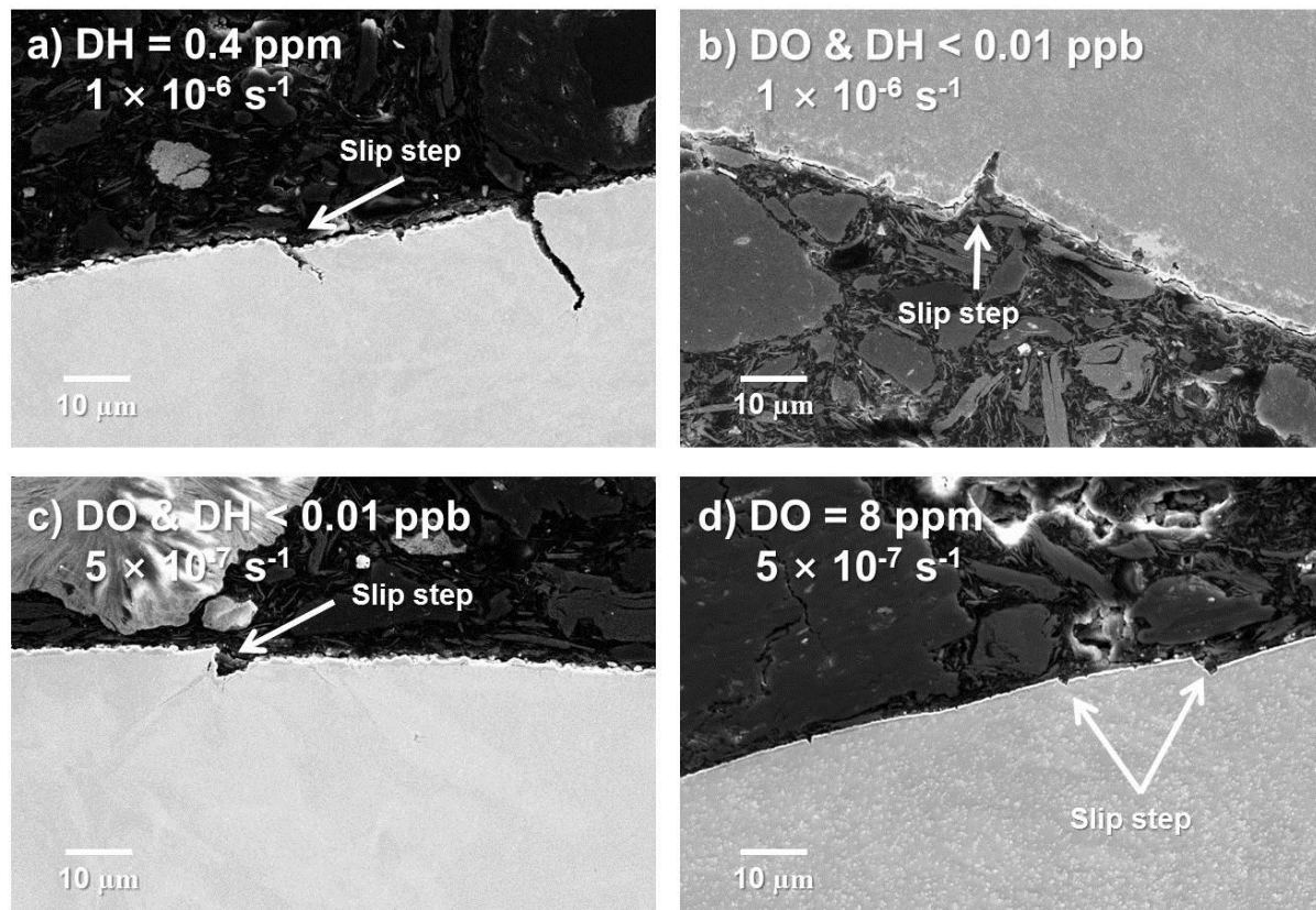
Fig. 4.24 Cross-sectional crack observation formed on SUS316L at lower strain rate of 1 \times 10^{-6} \text{ s}^{-1} or 5 \times 10^{-7} \text{ s}^{-1} in SCPW with a) DH 0.4 ppm, b & c) deaerated and d) DO 8 ppm.
