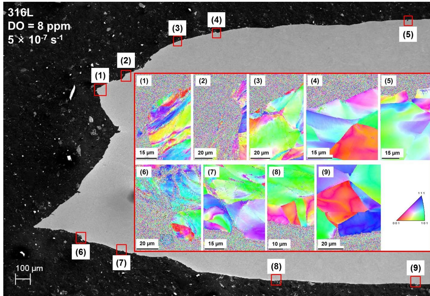
Fig. 4.18 EBSD analysis results of cracks on SUS316L after SSRT at lower strain rate of 5 \times 10^{-7} \text{ s}^{-1} in SCPW with 8 ppm dissolved oxygen.
