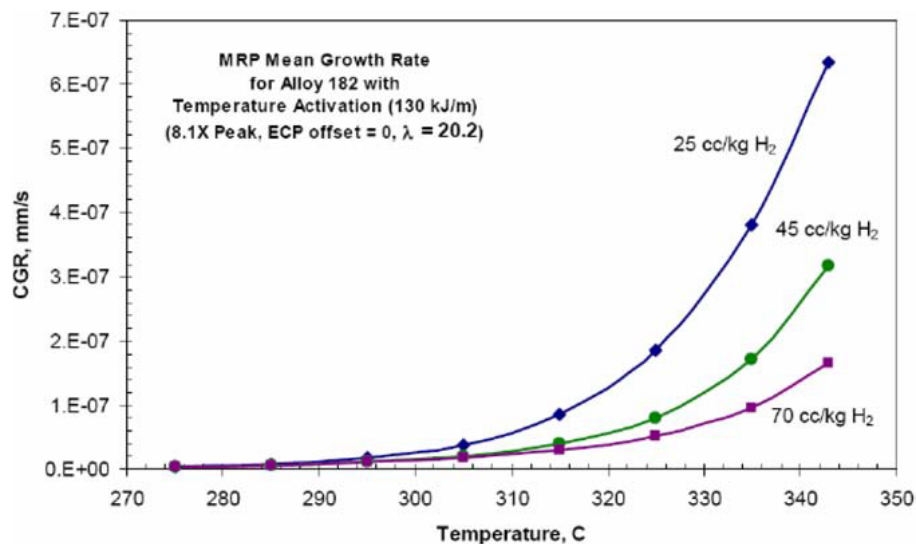
Fig. 2.12. Effect of temperature on PWSCC crack growth rate for alloy 182 [32].
