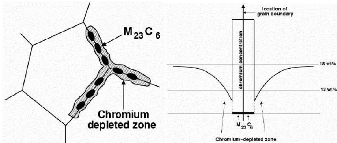
Fig.4.20 Schematic illustration of grain boundary chromium carbides precipitation and corresponding Cr profile. Chromium-depleted zones adjacent to grain boundaries are susceptible to intergranular corrosion [26]
