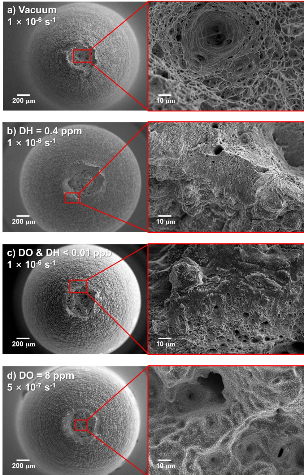
Fig. 4.7 Fracture surface of SUS316L austenitic stainless steel after SSRT at lower strain rate of 1 \times 10^{-6} \text{ s}^{-1} or 5 \times 10^{-7} \text{ s}^{-1} in a) vacuum, b) SCPW with DH 0.4 ppm, c) deaerated SCPW (DO & DH < 0.01 ppb) and d) SCPW with DO 8 ppm.
