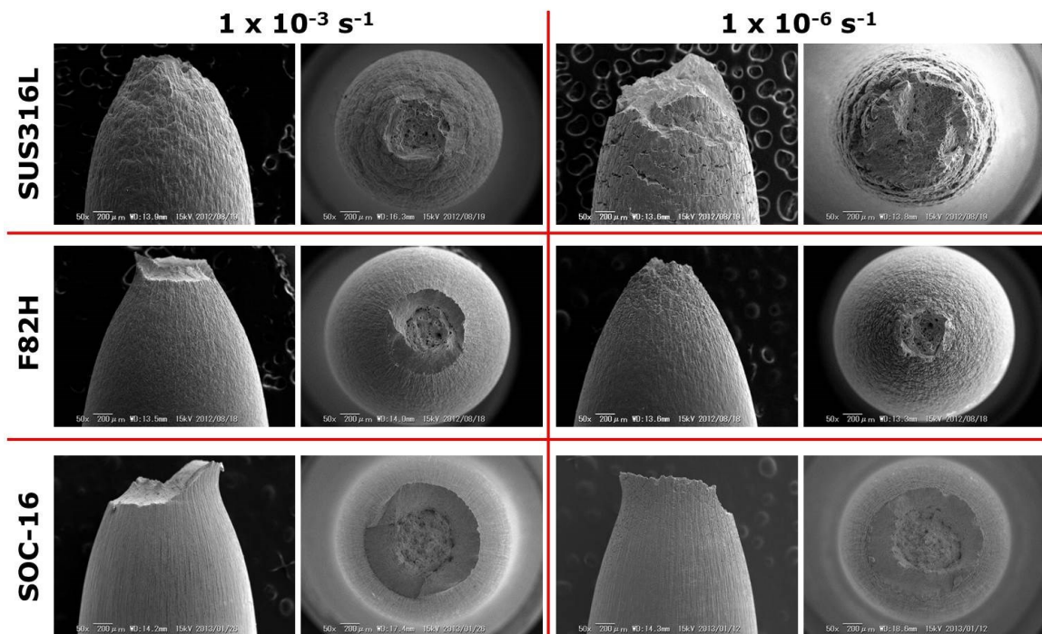
Fig. 5.4. Fracture surface and gauge section of the round bar specimen after SSRT in SCPW at higher strain rate ( 1 \times 10^{-3} \text{ s}^{-1} ) and lower strain rate ( 1 \times 10^{-6} \text{ s}^{-1} )
