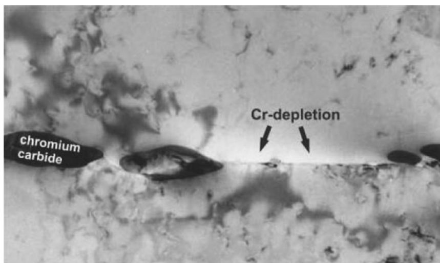
Fig 2.9 Transmission electron microscope (TEM) image showing Cr carbide precipitates along a grain boundary and the zone of Cr-depletion [27]
