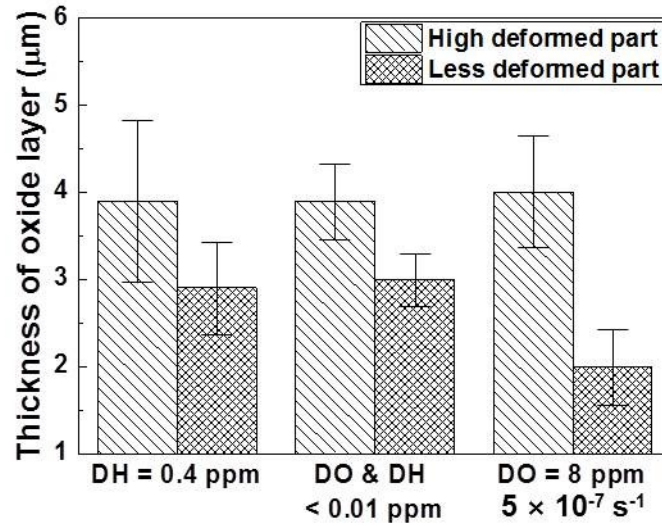
Fig. 3.7. Oxide layer thickness of highly deformed necking portion and less deformed gage portion after SSRT at lower strain rate of 1 \times 10^{-6} \text{ s}^{-1} or 5 \times 10^{-7} \text{ s}^{-1}
