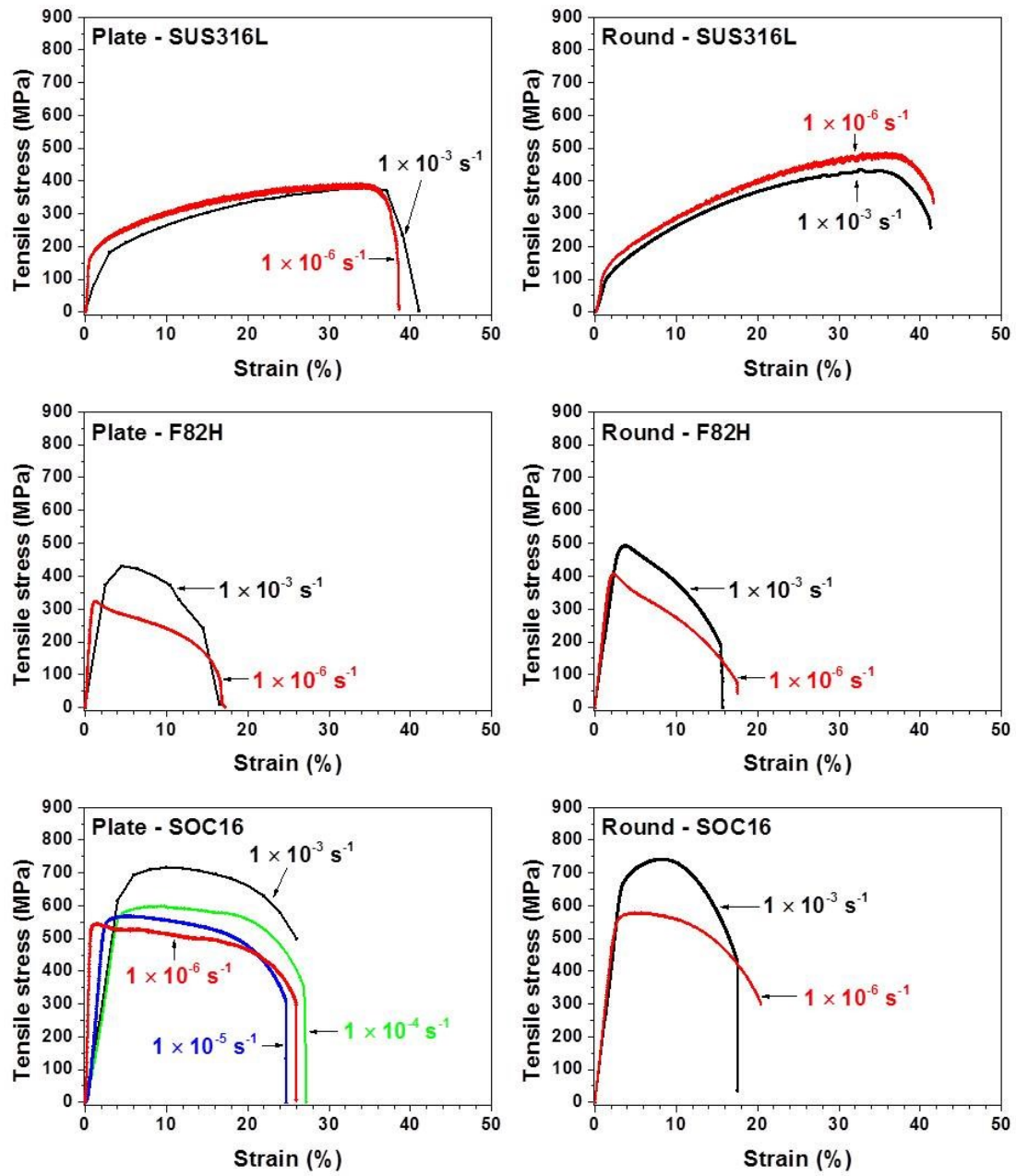
Fig 5.2. Stress-strain curves of SOC-16, F82H and SUS316L after SSRT in vacuum with different specimen morphology.
