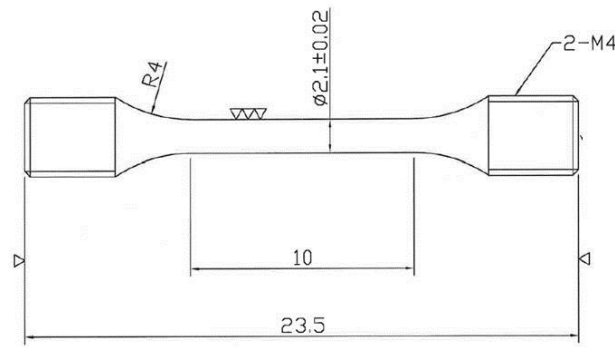
Fig. 3.1. The geometry of tensile specimens for SSRT in SCPW
