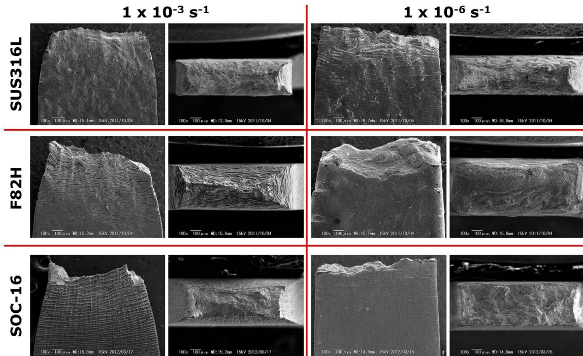
Fig. 5.3. Fracture surface and gauge section of the plate specimen after SSRT in SCPW at higher strain rate ( 1 \times 10^{-3} \text{ s}^{-1} ) and lower strain rate ( 1 \times 10^{-6} \text{ s}^{-1} )
