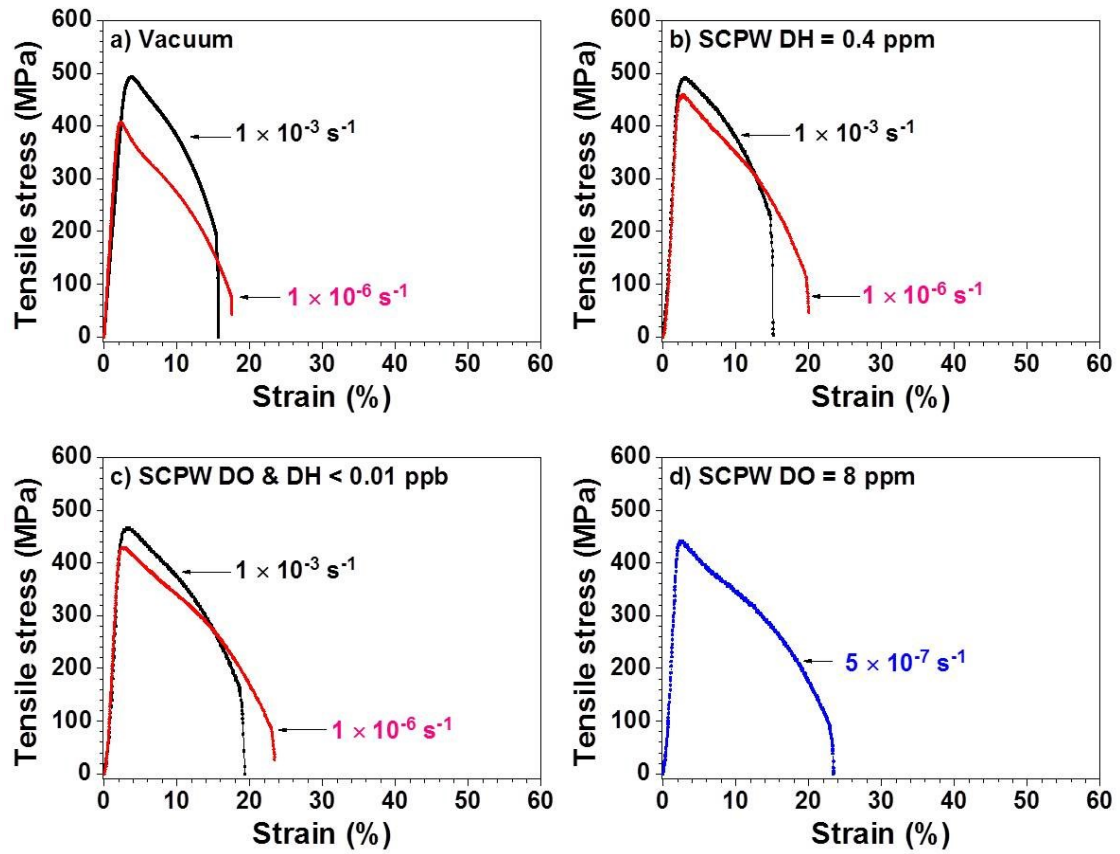
Fig. 4.2 SSRT stress-strain curves for F82H ferritic/martensitic steel as a function of different strain rate at each environment of a) vacuum, b) SCPW DH =0.4 ppm, c) SCPW DO & DH < 0.01 ppb (deaerated) and d) SCPW DO = 8 ppm
