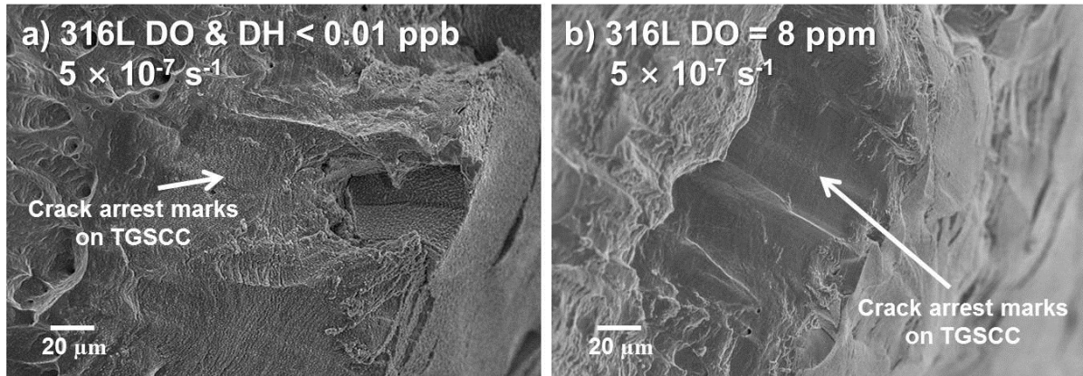
Fig. 4.23 Fracture surface of SUS316L austenitic stainless steel after SSRT at lower strain rate of 5 \times 10^{-7} \text{ s}^{-1} in (a) deaerated SCPW (DO & DH < 0.01 ppb) and (b) SCPW with DO 8 ppm.
