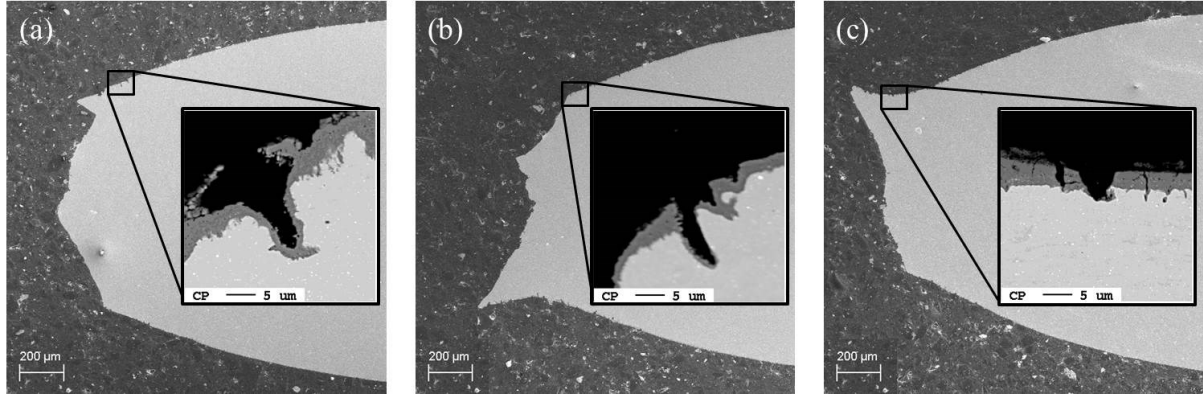
Fig. 3.9. Cross-sectional SEM images of specimens showing cracks after SSRT at lower strain rate in SCPW. (a : DH 0.4 ppm - 1 \times 10^{-6} \text{ s}^{-1} , b : DO & DH < 0.01 ppm - 1 \times 10^{-6} \text{ s}^{-1} , c : DO 8.0 ppm - 5 \times 10^{-7} \text{ s}^{-1} ,)
