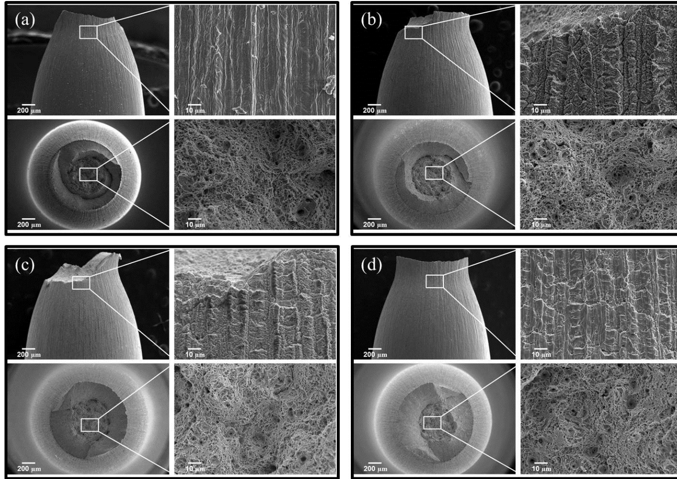
Fig. 3.4. SEM images of fracture surface and gauge section of the ODS steel after SSRT at a higher strain rate of 1 \times 10^{-3} \text{ s}^{-1} . (a : vacuum, b : SCPW with DH 0.4 ppm, c : SCPW with DO & DH < 0.01 ppm, d : SCPW with DO 8.0 ppm)
