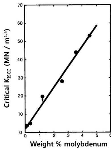
Fig. 4.26 The relationship between molybdenum contents and critical K ISCC of CrNiMo steel with 15.5-21%Ni 22%Cr in aerated NaCl solution at 105 °C
