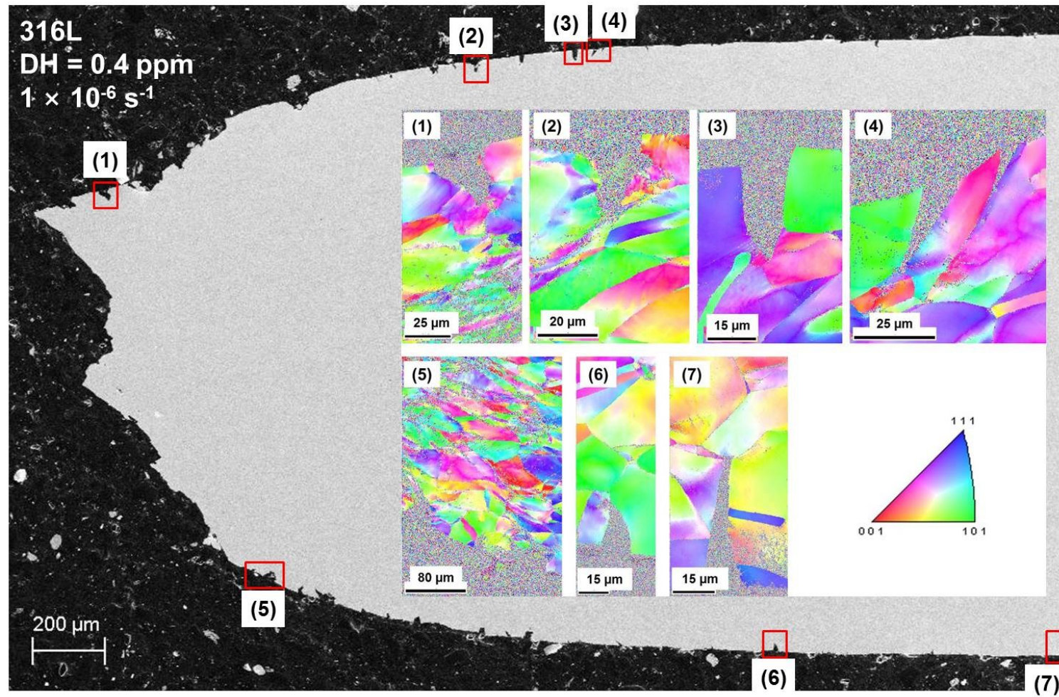
Fig. 4.15 EBSD analysis results of cracks on SUS316L after SSRT at lower strain rate of 1 \times 10^{-6} \text{ s}^{-1} in SCPW with 0.4 ppm dissolved hydrogen.
