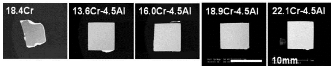
Fig. 2.1. The appearance of ODS steel specimens after corrosion test in LBE solved with 10^{-6} wt.%O 2 for 1 \times 10^4 h at 923 K.
