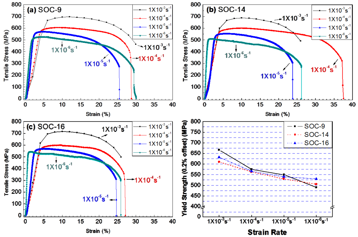
Fig. 6.1 Tensile test results of steady strain rate test for ODS steels at 773K in a vacuum at different strain rates ranging from 1 \times 10^{-3} \text{ s}^{-1} to 1 \times 10^{-6} \text{ s}^{-1} : (a) SOC-9, (b) SOC-14, (c) SOC-16, and (d) yield stress of ODS steels as a function of strain rate
