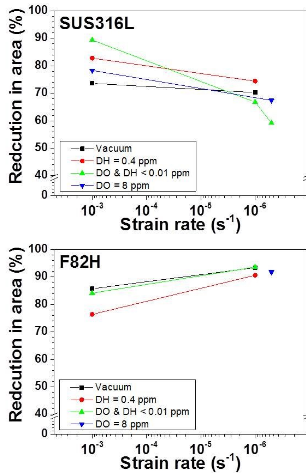
Fig 4.3. Reduction in area of SUS316L and F82H after fracture by SSRT.
