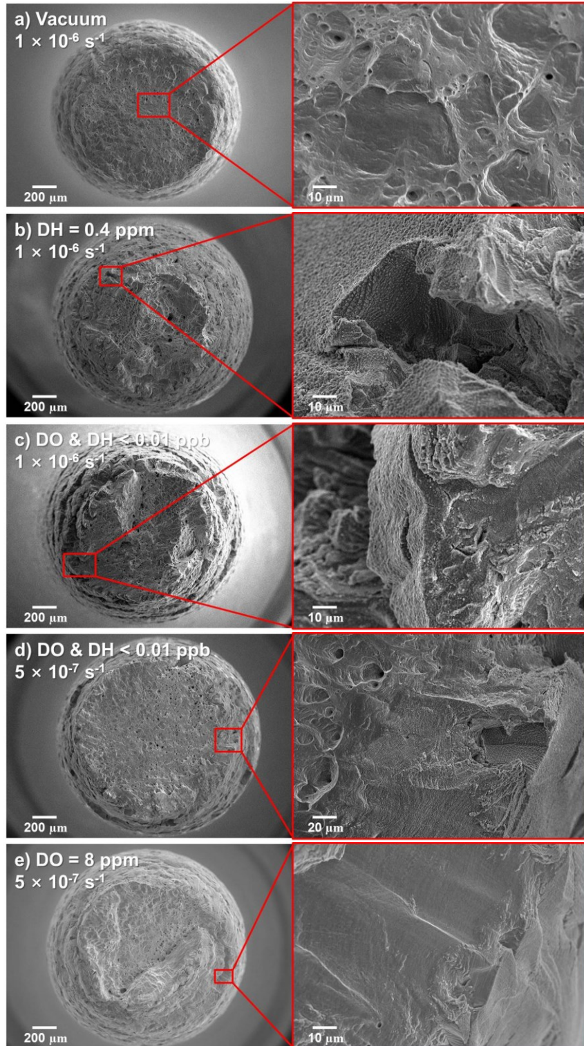
Fig. 4.6 Fracture surface of SUS316L austenitic stainless steel after SSRT at lower strain rate of 1 \times 10^{-6} \text{ s}^{-1} or 5 \times 10^{-7} \text{ s}^{-1} in (a) vacuum, (b) SCPW with DH 0.4 ppm, (c, d) deaerated SCPW (DO & DH < 0.01 ppb) and (e) SCPW with DO 8 ppm.
