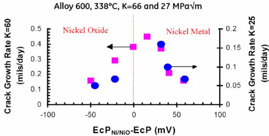
Fig. 2.11. Crack growth rate for alloy 600 in simulated PWR environment at 338 °C [32].
