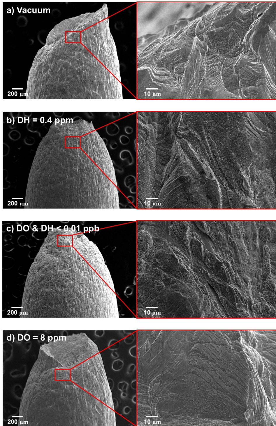
Fig. 4.8 Specimen side surface of SUS316L austenitic stainless steel after SSRT at higher strain rate of 1 \times 10^{-3} \text{ s}^{-1} in a) vacuum, b) SCPW with DH 0.4 ppm, c) deaerated SCPW (DO & DH < 0.01 ppb) and d) SCPW with DO 8 ppm.
