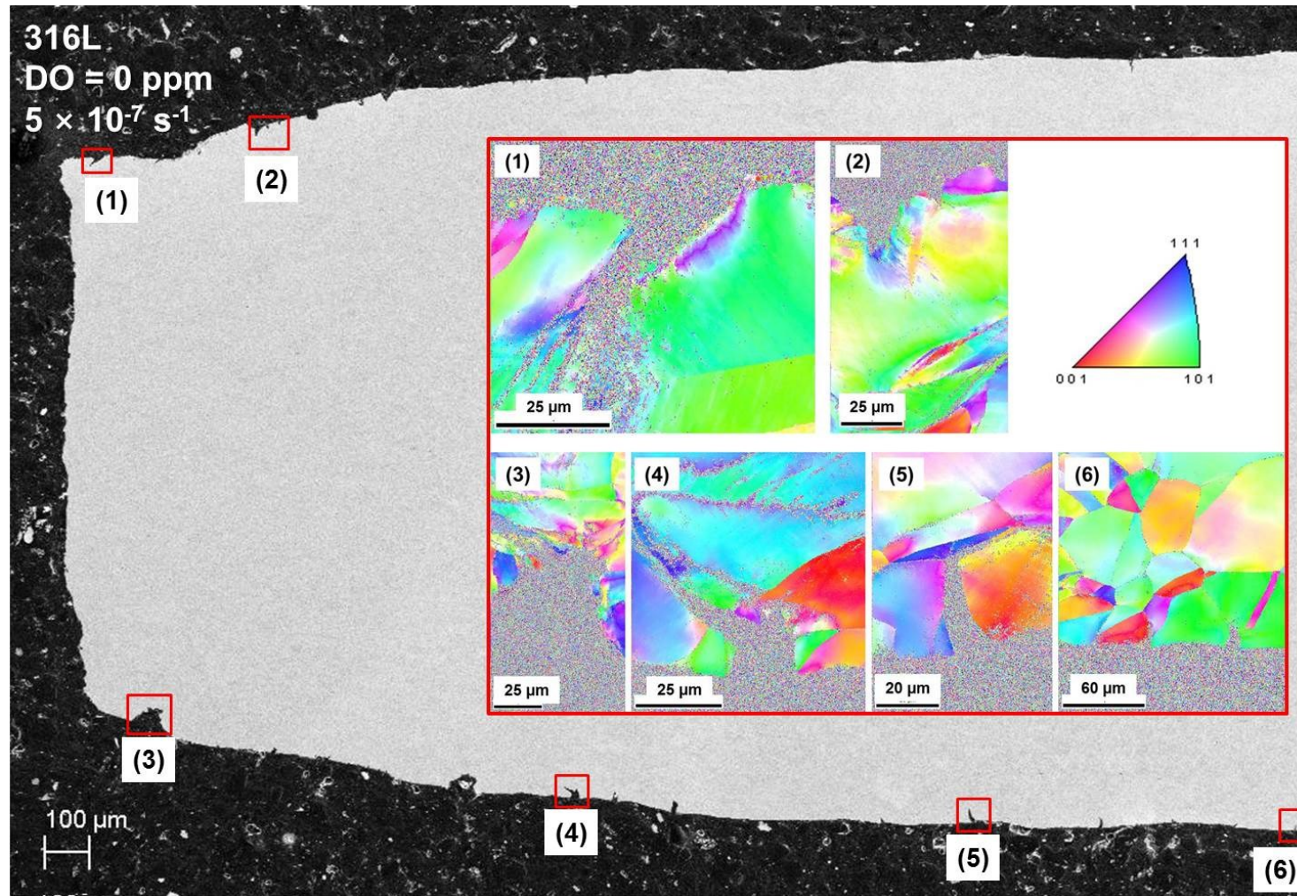
Fig. 4.17 EBSD analysis results of cracks on SUS316L after SSRT at lower strain rate of 5 \times 10^{-7} \text{ s}^{-1} in deaerated SCPW (DO & DH < 0.01 ppm)
