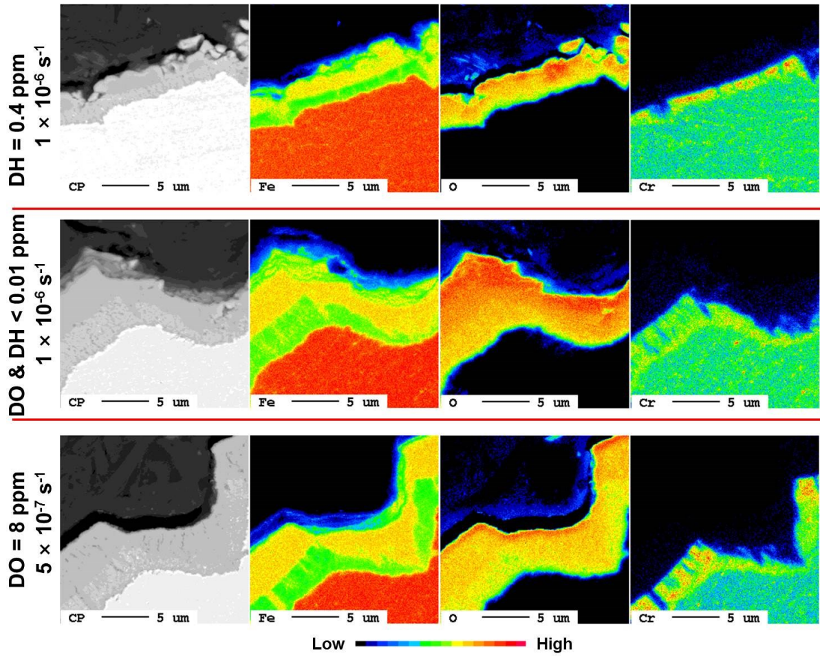
Fig. 4.13 EPMA analysis results of cracks on F82H after SSRT at lower strain rate of 1 \times 10^{-6} \text{ s}^{-1} or 5 \times 10^{-7} \text{ s}^{-1} in SCPW
