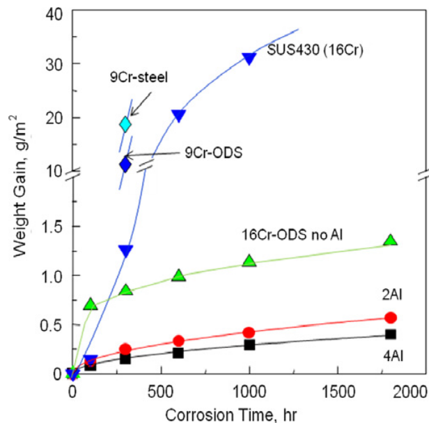
Fig. 2.2. Weight gain after corrosion tests in SCPW (773 K, 25 MPa) up to 1800 h.
