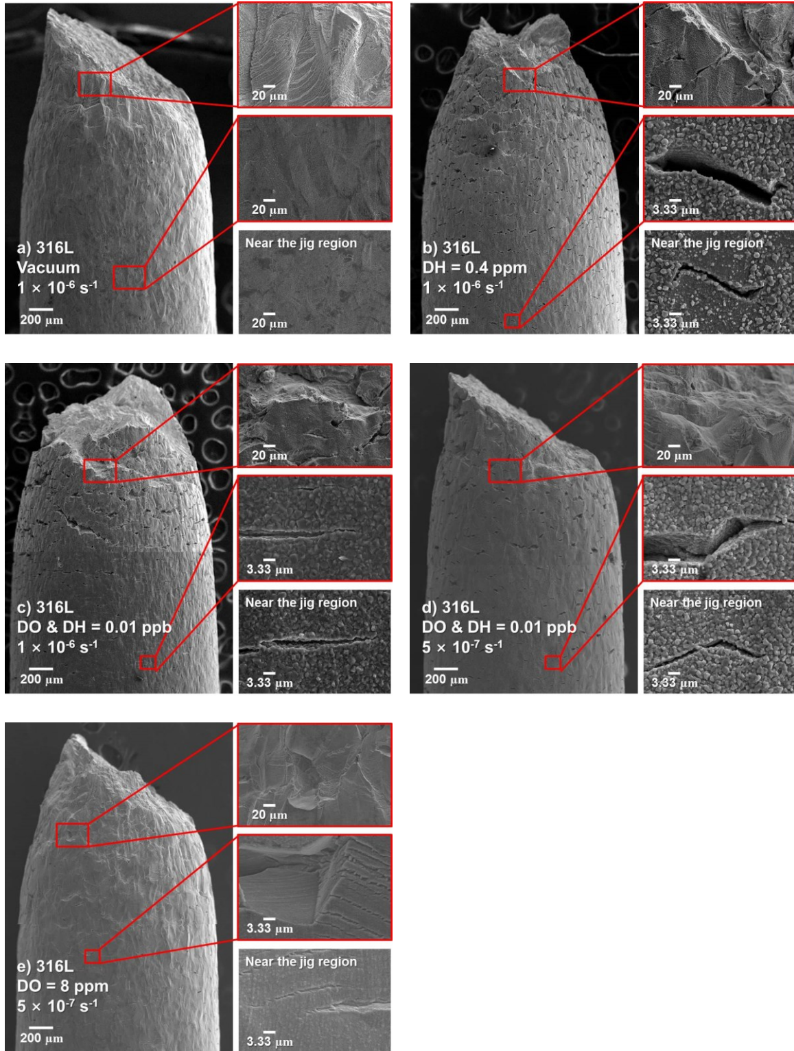
Fig. 4.10 Specimen side surface of SUS316L austenitic stainless steel after SSRT at lower strain rate of 1 \times 10^{-6} \text{ s}^{-1} or 5 \times 10^{-7} \text{ s}^{-1} in (a) vacuum, (b) SCPW with DH 0.4 ppm, (c, d) deaerated SCPW (DO & DH < 0.01 ppb) and (e) SCPW with DO 8 ppm.
