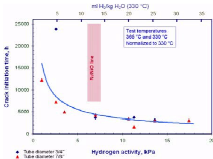
Fig. 2.13. The effect of hydrogen on initiation time. The data includes measurements at different temperatures normalized to the hydrogen partial pressure at 330 °C [33].
