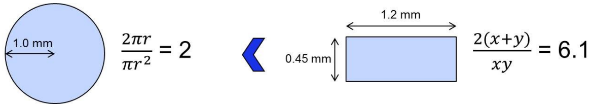
Fig. 5.6 The surface area ratio of the tested round bar and plate specimen.
