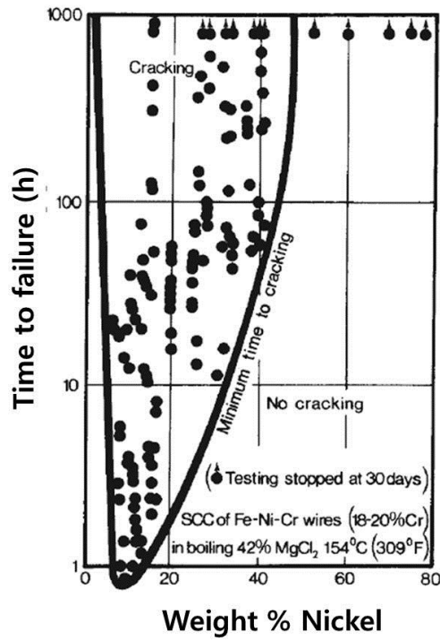
Fig. 4.25 Stress-corrosion cracking of iron-chromium-nickel wires in boiling 42% MgCl 2 at 154 °C [38]
