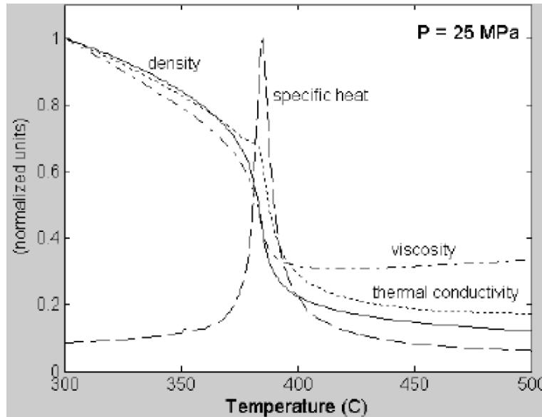
Fig. 2.7: Thermal variation of physical properties of water
