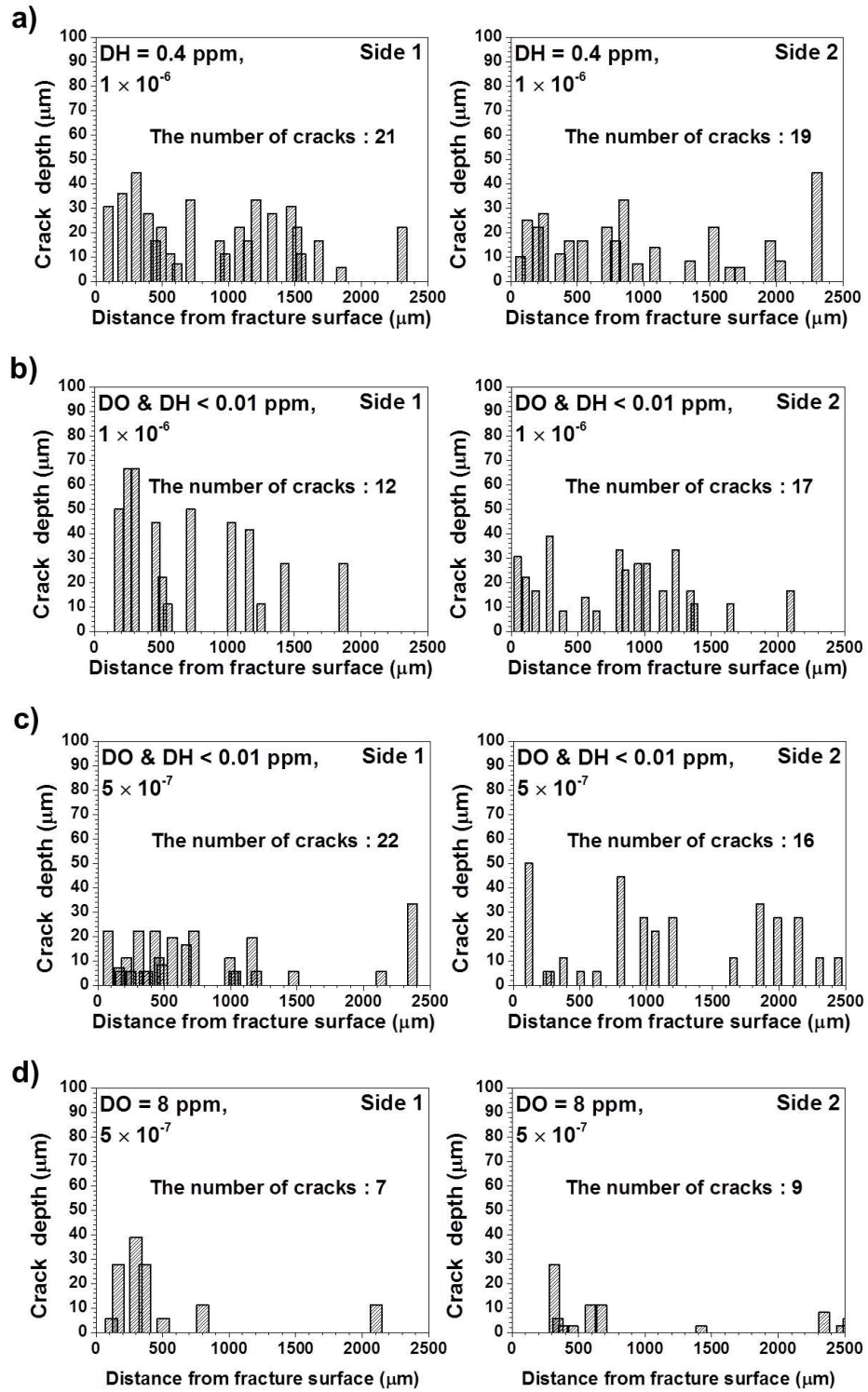
Fig. 4.14 The number and depth of SUS316L cracks according to the distance from fractured surface to the region 2.5 mm away from the fracture after SSRT deformed at lower strain rate of 1 \times 10^{-6} s -1 or 5 \times 10^{-7} s -1 in SCPW with a) DH 0.4 ppm, b & c) deaerated and d) DO 8 ppm. Side 1 and 2 are the bottom and top side of the cross sectional area of the specimens (refer to Fig. 4.15 – 4.18)
