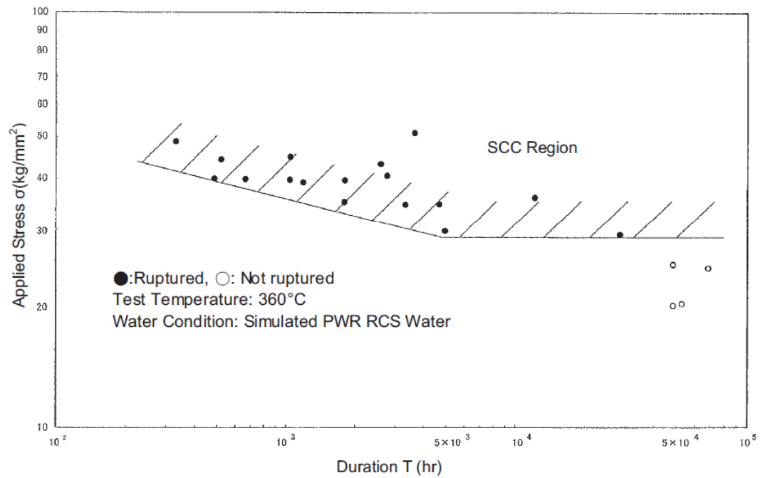
Fig. 2.16. Results of constant load PWSCC tests for alloy 132/82 weld metal.
