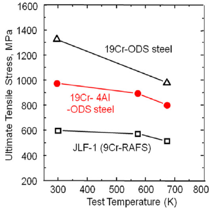
Fig. 2.3. The tensile strength of 19Cr-ODS steels with and without addition of Al as well as JLF-1 steel.
