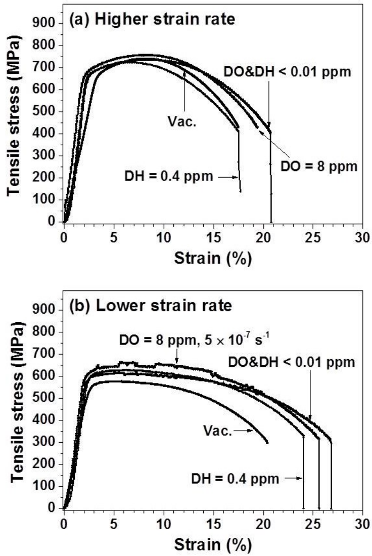
Fig. 3.2. SSRT stress-strain curves tested at (a) higher strain rate of 1 \times 10^{-3} \text{ s}^{-1} and (b) lower strain rate of 1 \times 10^{-6} \text{ s}^{-1} or 5 \times 10^{-7} \text{ s}^{-1} in vacuum and SCPW (DH = 0.4 ppm, DO & DH < 0.01 ppm and DO = 8 ppm)
