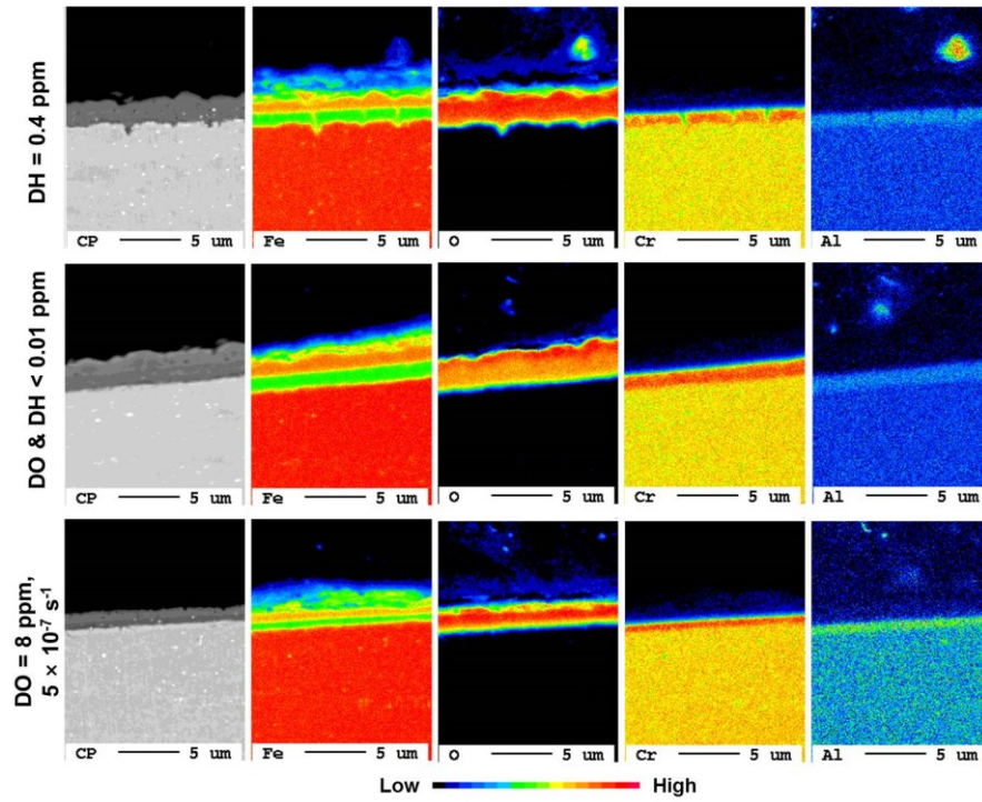
Fig. 3.6. EPMA analysis results of cross sectional area of the specimens after SSRT in SCPW at lower strain rate of 1 \times 10^{-6} \text{ s}^{-1} or 5 \times 10^{-7} \text{ s}^{-1} (scale shows the relative concentration).
