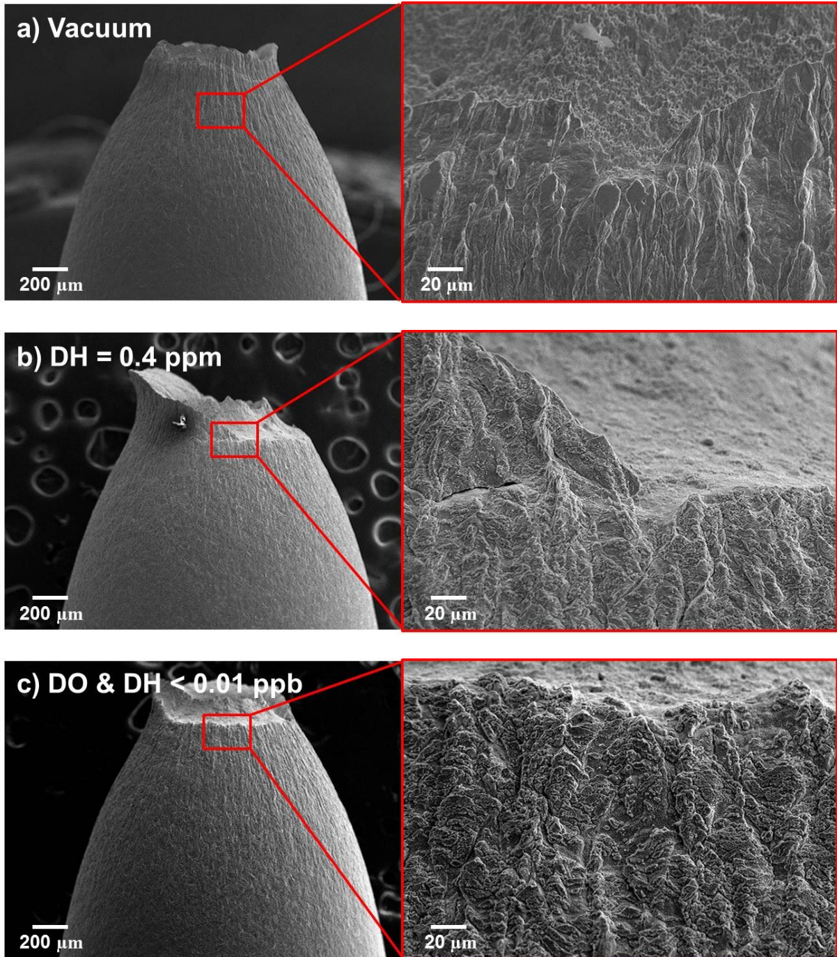
Fig. 4.9 Specimen side surface of F82H ferritic / martensitic steel after SSRT at higher strain rate of 1 \times 10^{-3} \text{ s}^{-1} in a) vacuum, b) SCPW with DH 0.4 ppm and c) deaerated SCPW (DO & DH < 0.01 ppb)
