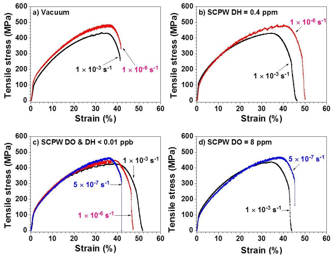
Fig. 4.1 SSRT stress-strain curves for SUS316L austenitic stainless steel as a function of different strain rate at each environment of a) vacuum, b) SCPW DH = 0.4 ppm, c) SCPW DO & DH < 0.01 ppb (deaerated) and d) SCPW DO = 8 ppm
