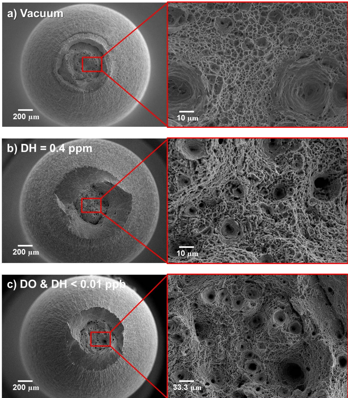
Fig. 4.5 Fracture surface of F82H ferritic / martensitic steel after SSRT at higher strain rate of 1 \times 10^{-3} \text{ s}^{-1} in a) vacuum, b) SCPW with DH 0.4 ppm and c) deaerated SCPW (DO & DH < 0.01 ppb)
