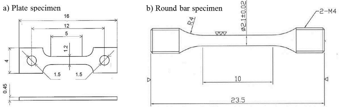
Fig 5.1. The geometry of tensile specimens for SSRT
