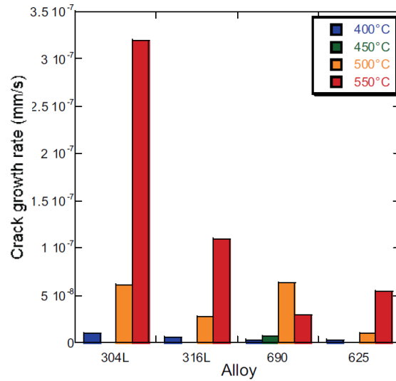
Fig. 2.18. Crack growth rate measured from cross sections of CERT samples for alloys 304L, 316L, 625 and 690 between 400 °C and 550 °C in deaerated SCW. [37]
