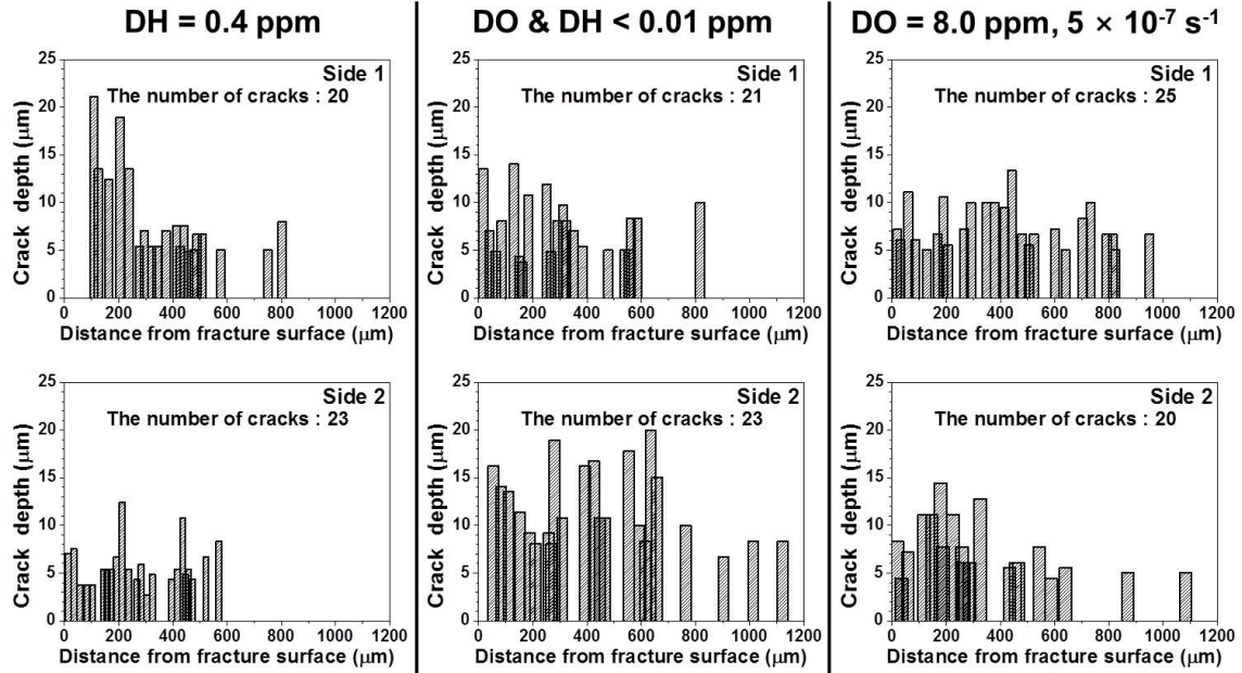
Fig. 3.8. The number and depth of cracks according to the distance from fractured surface after SSRT deformed at lower strain rate of 1 \times 10^{-6} \text{ s}^{-1} or 5 \times 10^{-7} \text{ s}^{-1} in SCPW. Side 1 and 2 are the bottom and top side of the cross sectional area of the specimens in Fig. 3.9
