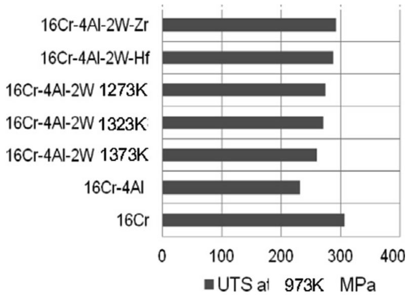
Fig. 2.4. Effects of extrusion temperature and addition of minor elements on the ultimate tensile stress (UTS) of 16Cr–4Al ODS steel at 973 K.
