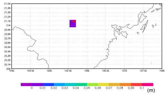
Fig.13 Spatial water conduction in inundation depths
