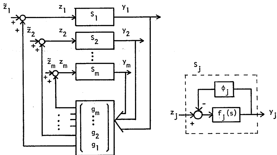
Fig. 1-2 Composite systems consisting of subsystems with nonlinear feedbacks.
