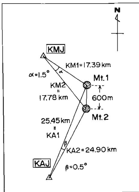
Fig. 2. Location of two quarry sites, Mt. 1 and Mt. 2, and two permanent stations, KMJ and KAJ.
