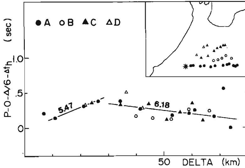
Fig. 6. (a) Time-distance relation for the group of A-D lines.
