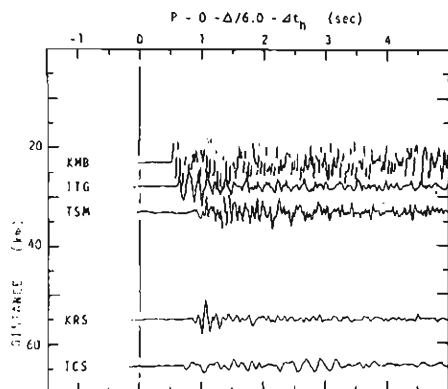
(e) Recorded seismograms arranged for E-line.
