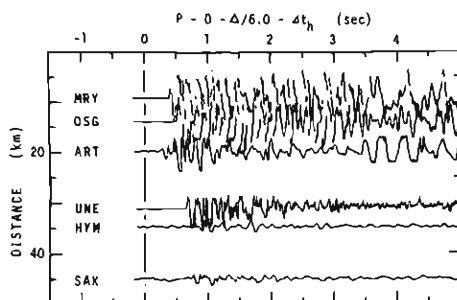
(h) Recorded seismograms arranged for H-line.
