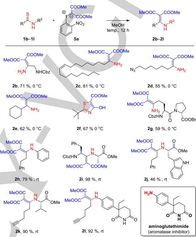
Figure 1. Substrate scope for synthesis of enaminones.
