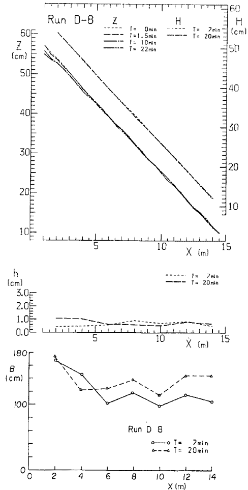
Fig. 13. Water surface and stream bed profiles and longitudinal changes in mean depth and water surface width in run D-8.
