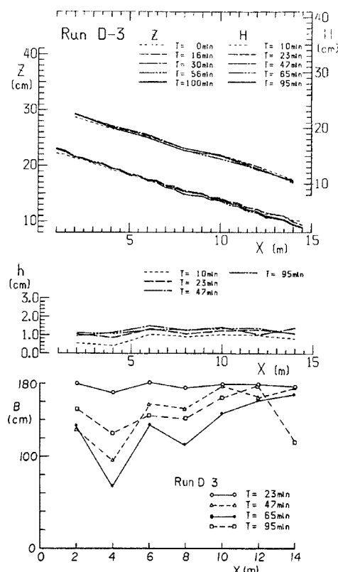
Fig. 15. Water surface and stream bed profiles and longitudinal changes in mean depth and water surface width in run D-3.
