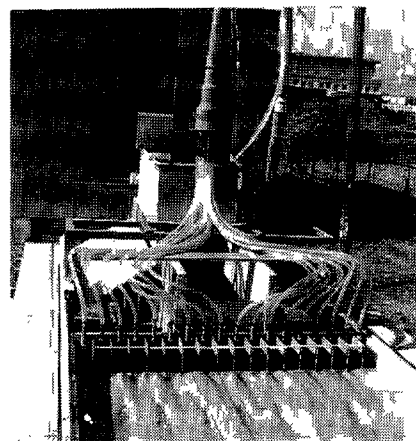
Photo. 1. Distributing device for water and sediment.
