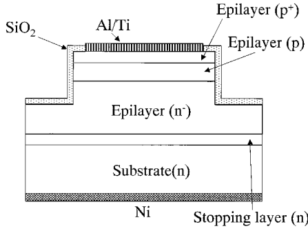
Fig. 1. Schematic view of SiC p-i-n diode.
