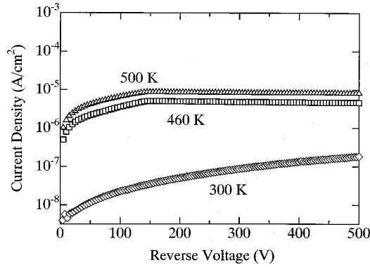
Fig. 4. Semi-logarithmic reverse J - V characteristics of SiC p-i-n diode at different temperatures.
