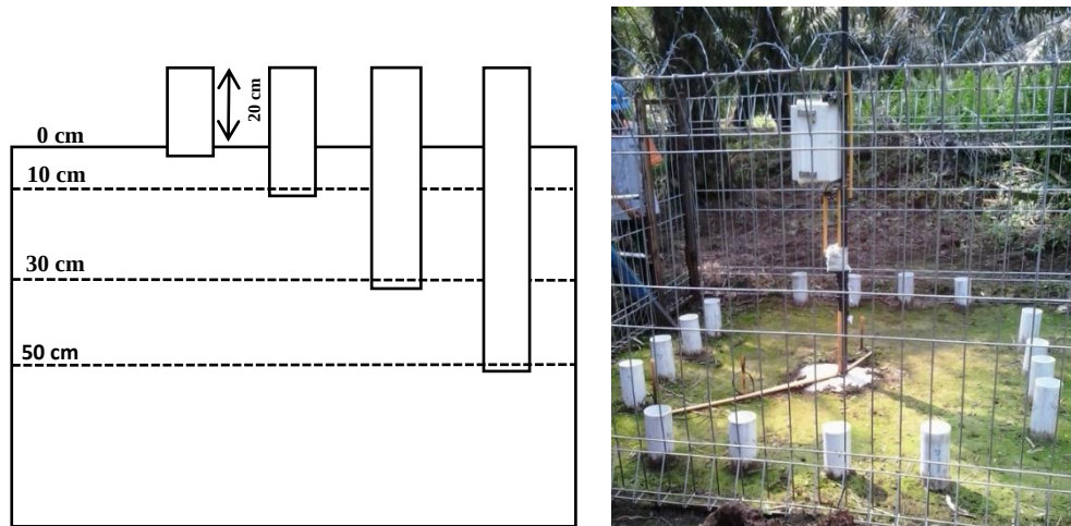
Figure 3. 1. Sketch of four chamber depth treatments of 0, 10, 30, and 50 cm with additional 20 cm length above the ground and 2 cm inserted into peat (left). Picture of the formation of 16 chambers, sensor device, and data logger installment in the site (right).
