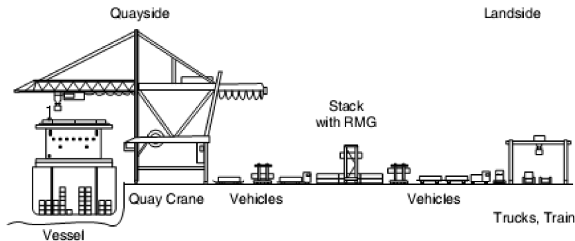
Figure 2: Typical layout of the container terminal [3].
