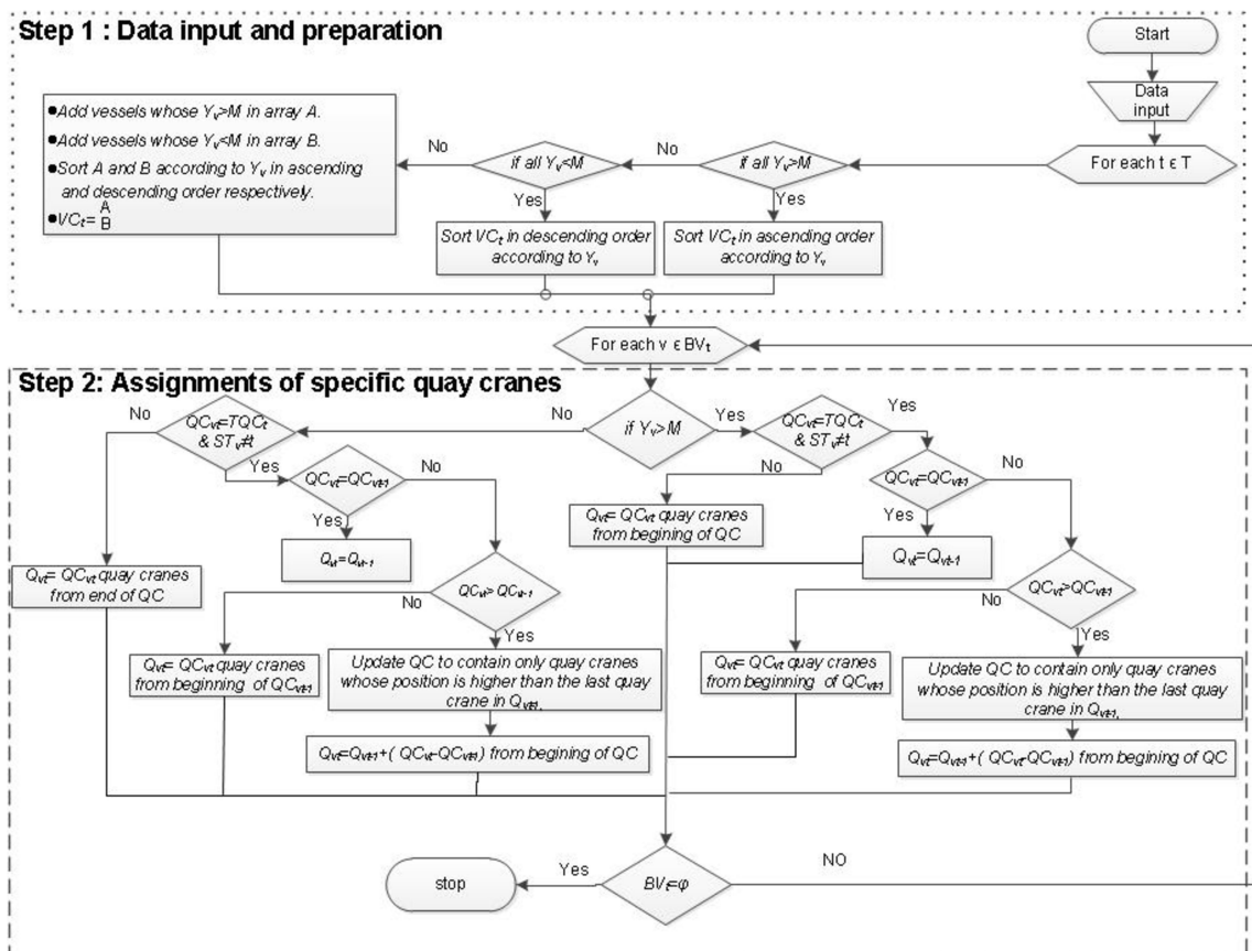
Figure 5: The detailed flow chart of the heuristic procedure
