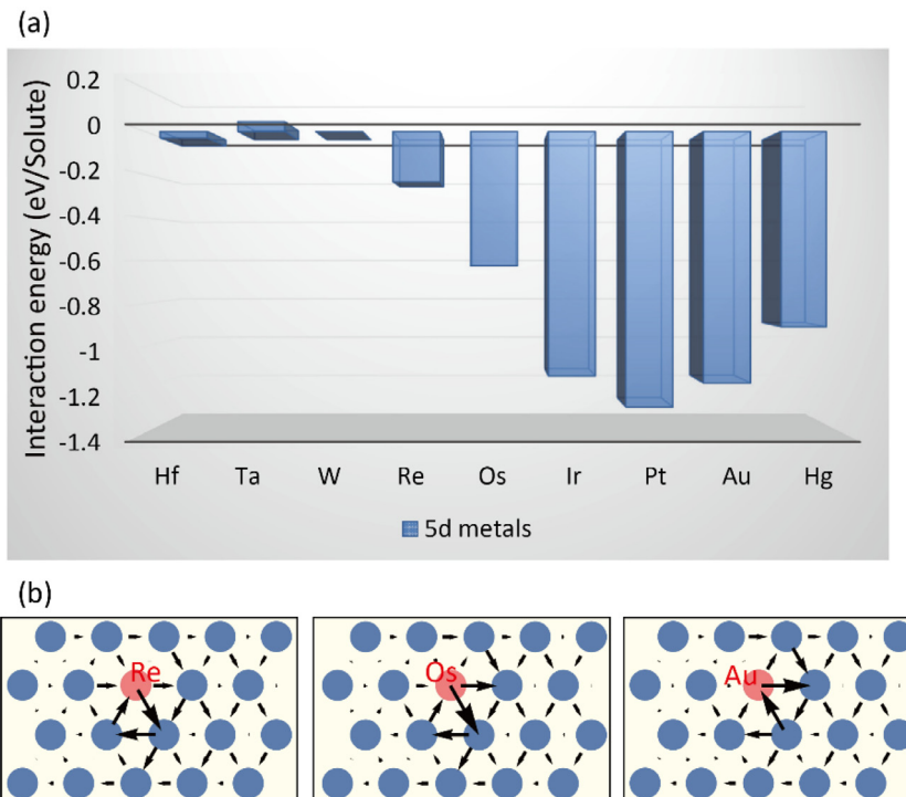
Fig. 3. Effects of different solutes on the dislocation core. (a) Interaction energies between the solutes and the dislocation for 1st nearest neighbor configuration after atomic relaxation. (b) DD maps for W-Re, W-Os, and W-Au.
