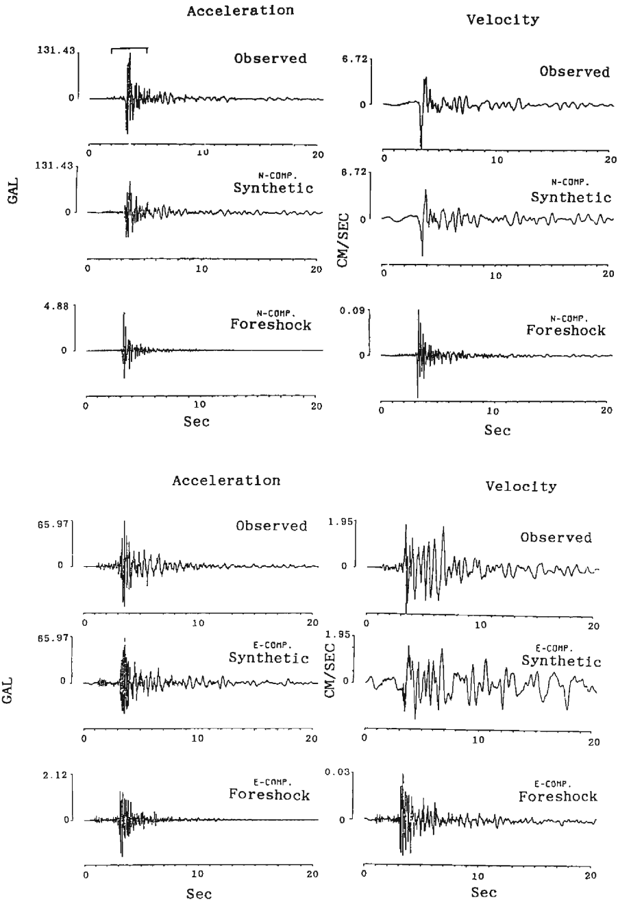
Fig. 7. Simulation at KR1 site. Upper : NS component, Lower : EW component. Left : Acceleration, Right : Velocity. From top to bottom : observed, synthetic and foreshock. (Note the different scale for the foreshock record).
