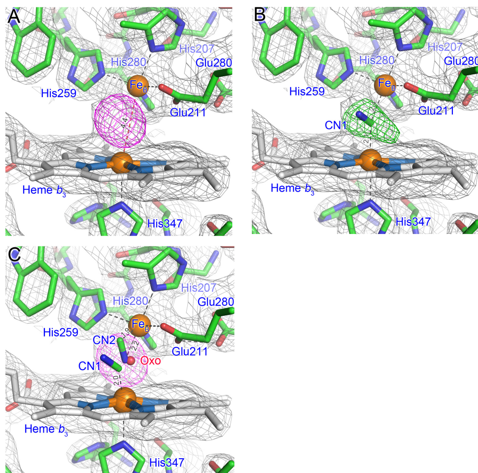
Figure 4. Electron density map of NO reduction site of the oxidized cyanide-bound form of P. aeruginosa cNOR. (A) F_o - F_c map at 8 \sigma (magenta) and 2F_o - F_c map contoured at 1.4 \sigma (gray mesh) indicate the binding of cyanide(s). (B) F_o - F_c map at 4.0 \sigma (green mesh) after the crystallographic refinement in which one cyanide was tentatively modeled. Residual density in F_o - F_c map indicates the presence of additional atoms. (C) Proposed model for the oxidized cyanide-bound form of cNOR shows the binding of two cyanide molecules to the binuclear active center with 80% occupancy. The remaining 20% was modeled as the oxygen atom (oxo) that bridges two Fe atoms in a resting state. The unbiased omit map (magenta mesh) and 2 F_o - F_c map (gray mesh) are contoured at 8.0 and 1.4 \sigma , respectively.
