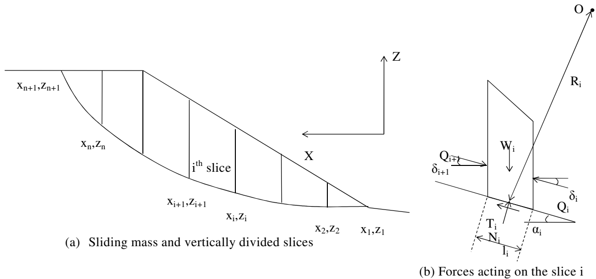
Fig. 2 Two dimensional general slip surface and forces acting on a typical slice
