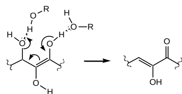
Fig. 11. A proposed inhibition mechanism for dehydration occurring during pyrolysis of a reducing sugar in polyether.
