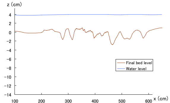
Fig. 5 Longitudinal profile of water surface and bed level along main channel (y=40cm) – Case 2.
