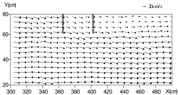
Fig. 8 Velocity field around groins in XY plane at z=2.0\text{cm} – Case 1 (experiment).
