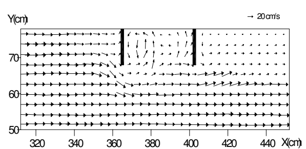
Fig. 9 Velocity field around groins in XY plane at z=2.0\text{cm} – Case 1 (simulation).
