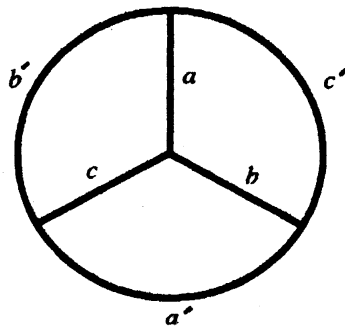
Figure 2 A fatgraph for the four-punctured sphere.
