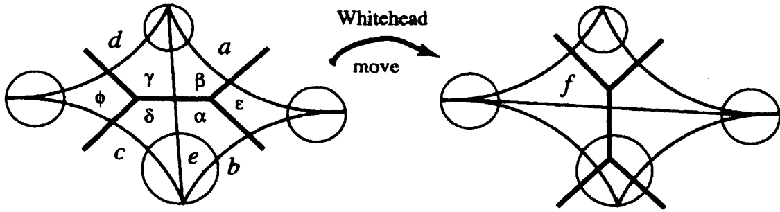
Figure 4 Standard notation for Whitehead moves.
