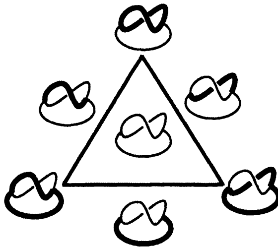
Figure 1 Screens for the once-punctured torus correspond to ideal vertices in the decomposition of P\tilde{T}(F_1^1) .
