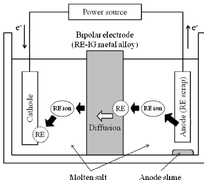
Figure 1. A new separation and recovery process of RE metals from scraps using molten salt and alloy diaphragm (1).
