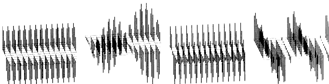
FIGURE 15. Here we show the projected versions of the eigenvectors in the previous figure, for use in comparing with the eigenfunctions of the smooth case considered in section 5. These projected versions are made the same way as in Figure 12.
