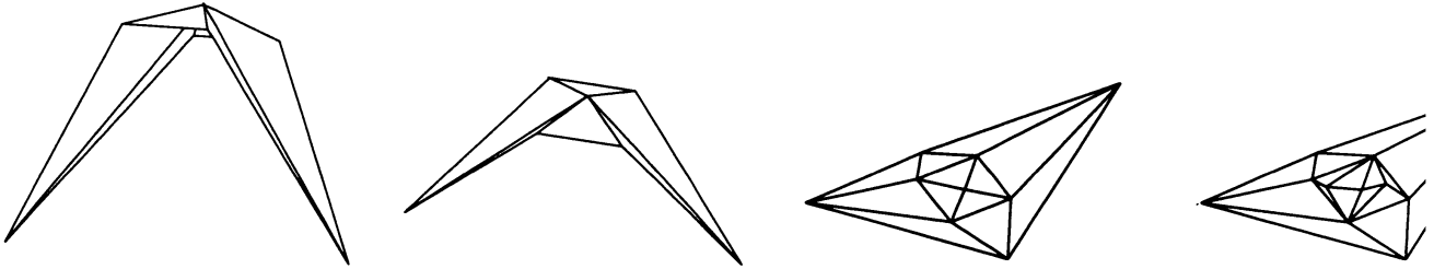
FIGURE 2. Two views on the left-hand side of a surface that defines the maximum principle, and two discrete minimal surfaces on the right-hand side with boundary vertices (x, 0, z_1) , (-x, 0, z_1) , (0, y, z_2) , and (0, -y, z_2) in \mathbb{R}^3 . These two surfaces on the right have the same trace in \mathbb{R}^3 but have different simplicial structures, and a surprising feature of these examples is that the innermost triangles form a square, regardless of the values of x, y, z_1 \neq z_2 .
