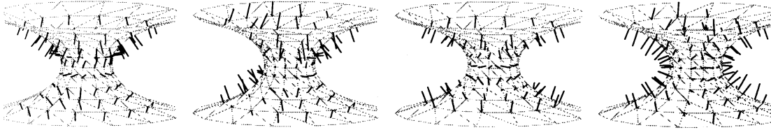
FIGURE 14. One-third of the eigenvectors are approximately perpendicular to the surface. For example, here we show the \mathbb{R}^{3n} -eigenvector fields associated to the eigenvalues \lambda_{147} , \lambda_{171} , \lambda_{204} , and \lambda_{210} .
