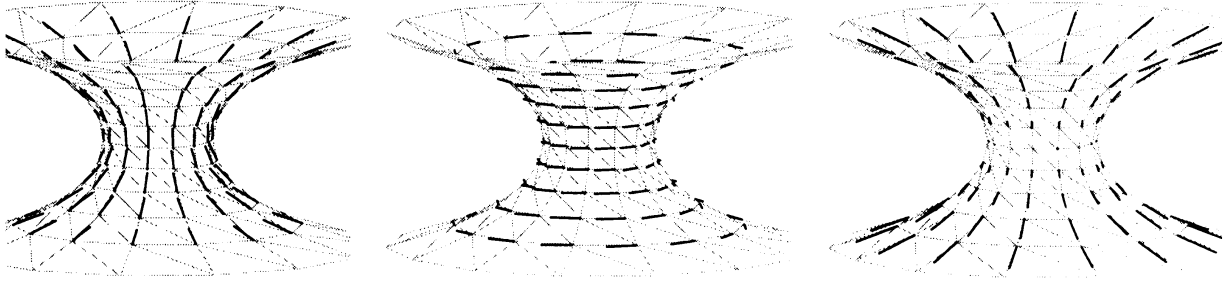
FIGURE 13. Two-thirds of the eigenvectors are approximately tangential to the surface. For example, here we show the \mathbb{R}^{3n} -eigenvector fields associated to the eigenvalues \lambda_1 , \lambda_2 , and \lambda_3 (whose values are just slightly greater than 0).
