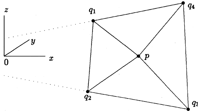
FIGURE 6. The construction in Lemma 3.3.
