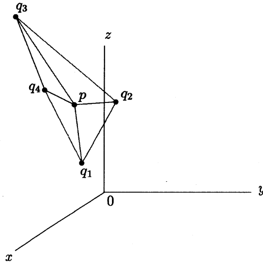
FIGURE 4. The construction in Lemma 3.1.
