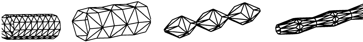
FIGURE 7. Discrete analogues of cylinders and Delaunay surfaces.
