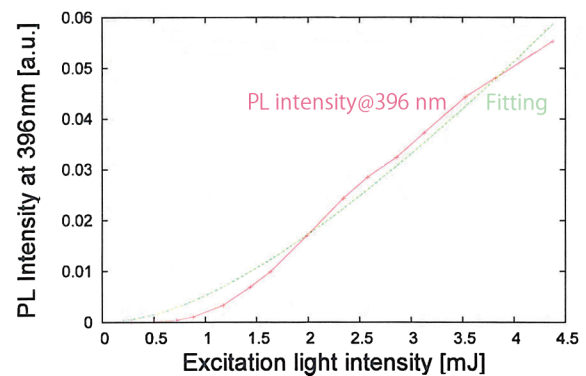
FIG. 2 Photoluminescence intensity at 396 nm in FIG. 1 and fitting by Eq. 1 versus excitation light intensity [B3].
