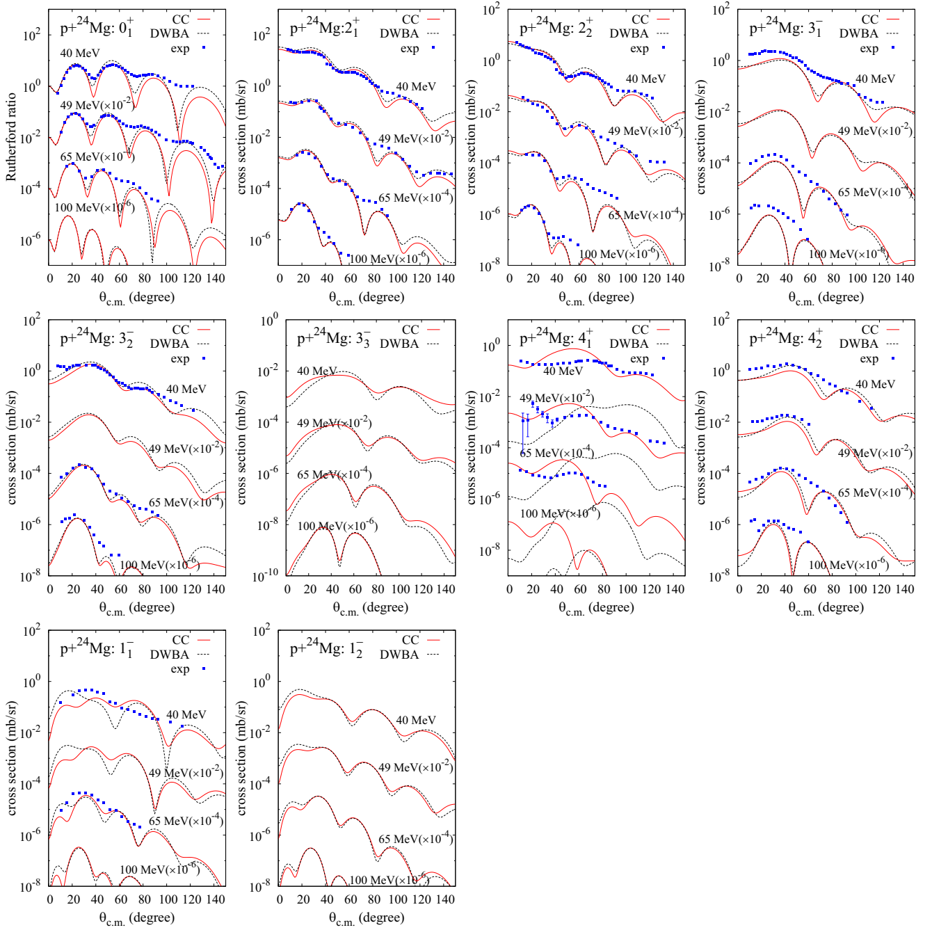
FIG. 8. Cross sections of proton scattering off ^{24}\text{Mg} at incident energies of E_p = 40, 49, 65 , and 100 MeV, as calculated with MCC+AMD (solid lines with label “CC”) and DWBA (dotted lines with label “DWBA”). For the 4_1^+ state, the DWBA cross sections are two orders smaller than the CC cross sections. Experimental data are cross sections at E_p = 40 MeV [15,16], 49 MeV [13], 65 MeV [17,70], and 100 MeV [18,70].
