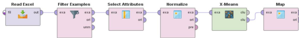
Figure 1. Clustering process
