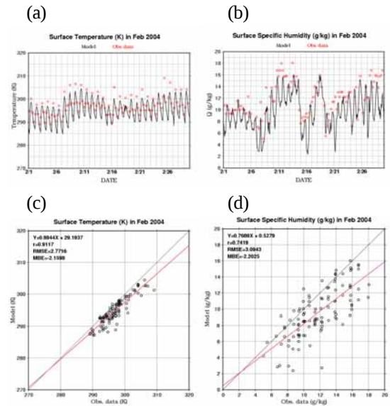
Fig.7 Model comparison with observation data in February 2004 at Jeddah. Upper panels mean time series for (a) temperature and (b) specific humidity at 2m height on the ground; solid lines mean model results and circles show observation data, and lower panels represent correlations for (c) temperature and (d) specific humidity, with regression lines.
