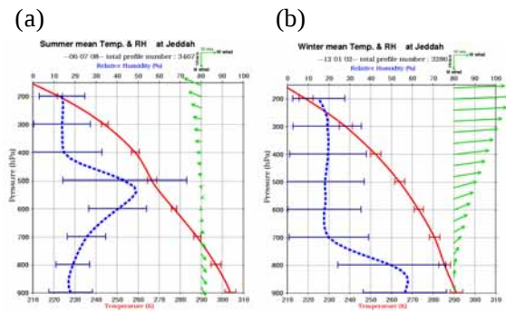
Fig. 2 Mean profile of temperature, RH, and wind in (a) summer and (b) winter at Jeddah.
