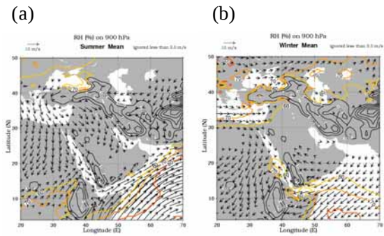
Fig. 3 Seasonal distribution of RH and wind in (a) summer and (b) winter on 900hPa.
