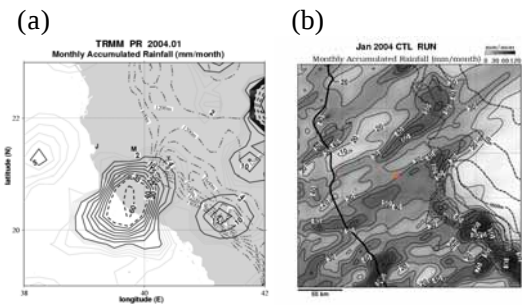
Fig.6 Rainfall distribution in January 2004 by (a) TRMM and (b) model result.
