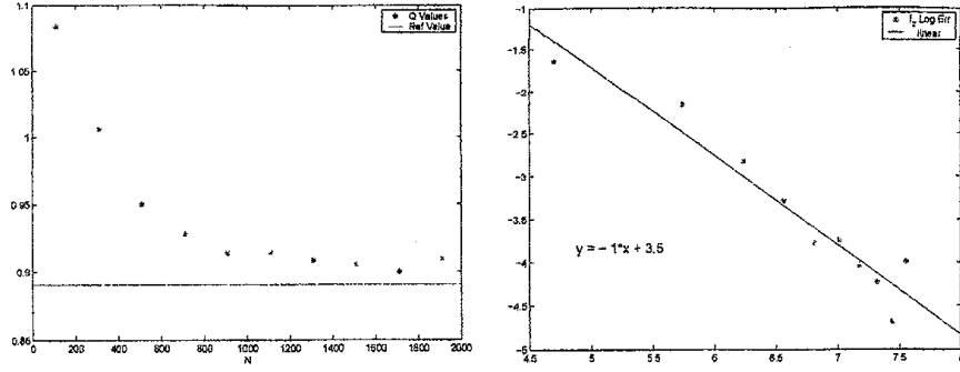
Figure 2b : dim3 - : Convergence and Convergence Rate (in a ln-scale) of \hat{\Pi}_n \phi_2 as N grows, for n = 15 and \phi_2(x) = |x|^2 .
