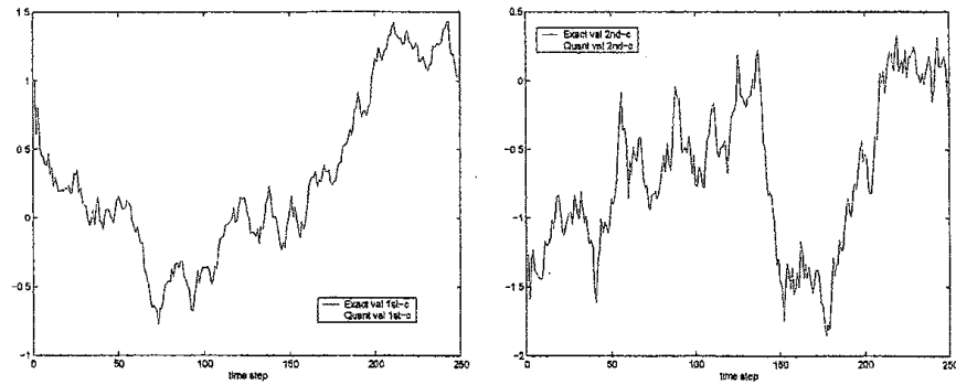
Figure 3 : dim 2 - : Error dependence of \hat{\Pi}_n \phi as n grows, for \bar{N} = 600 , \phi(x) = x_1 and \phi(x) = x_2 .
