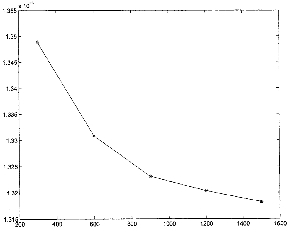
Figure 5 : Filter error convergence as N grows
