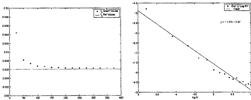
Figure 1c : dim1 - : Convergence and Convergence Rate (in a ln-scale) of \hat{\Pi}_n \phi_3 as N grows, for n = 15 and \phi_3(x) = \exp(-|x|) .
