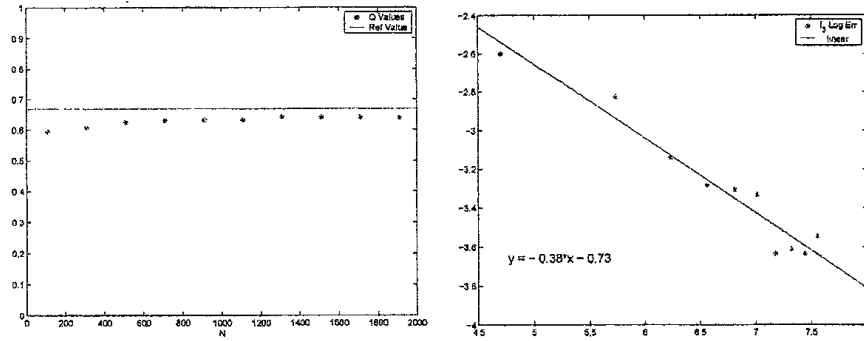
Figure 2c : dim3 - : Convergence and Convergence Rate (in a ln-scale) of \hat{\Pi}_n \phi_3 as N grows, for n = 15 and \phi_3(x) = \exp(-|x_3|) .
