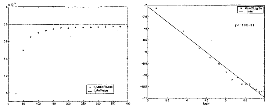
Figure 1b : dim1 - : Convergence and Convergence Rate (in a ln-scale) of \hat{\Pi}_n \phi_2 as N grows, for n = 15 and \phi_2(x) = x^2 .
