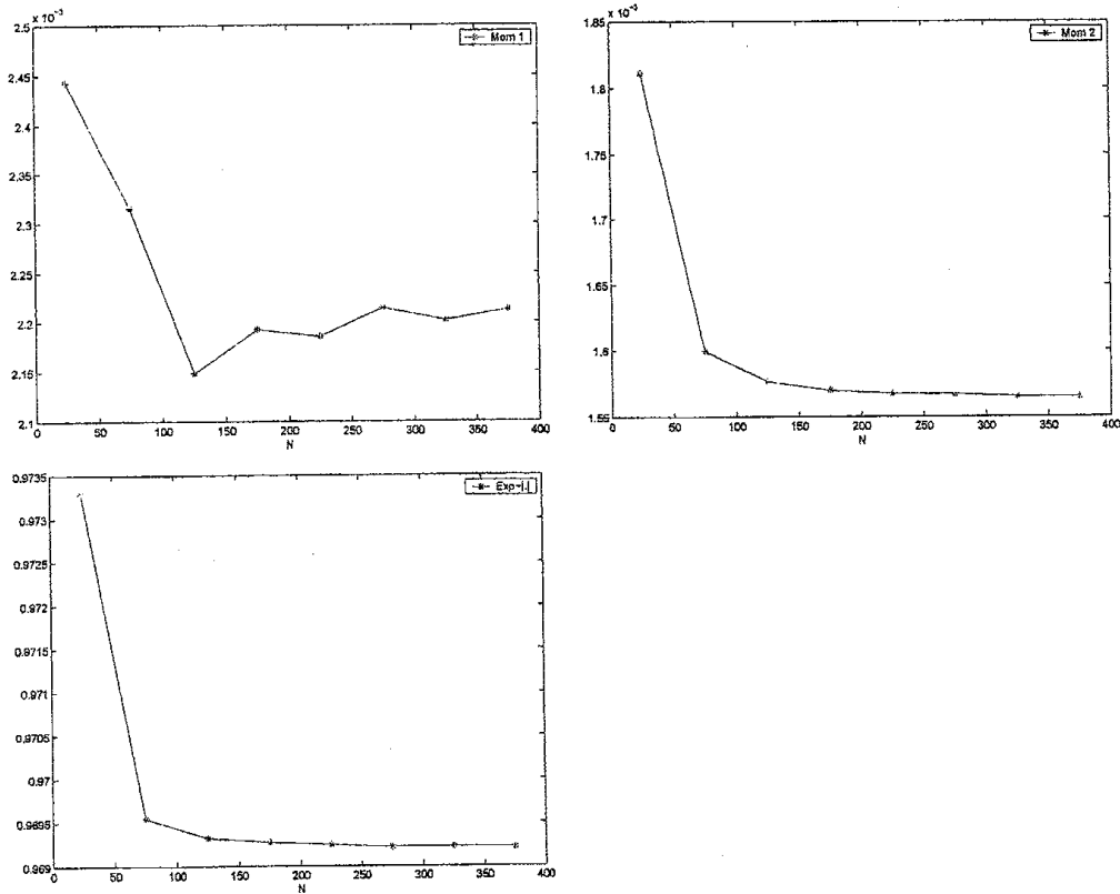
Figure 4 : SV model : filter values of \hat{\Pi}_n \phi at fixed n as \bar{N} grows, for \phi(x) = x , |x|^2 , and \exp(-|x|) .
