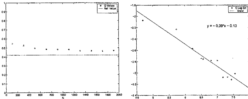
Figure 2a : dim3 - : Convergence and Convergence Rate (in a ln-scale) of \hat{\Pi}_n \phi_1 as N grows, for n = 15 and \phi_1(x) = x_3 .
