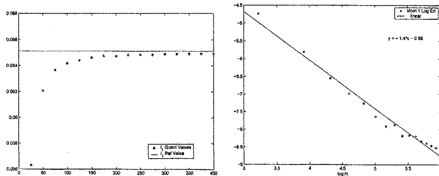
Figure 1a : dim1 - : Convergence and Convergence Rate (in a ln-scale) of \hat{\Pi}_n \phi_1 as N grows, for n = 15 and \phi_1(x) = x .
