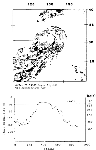
Fig. 9 (a) Same as Fig. 2 (a), except for 09JST Sept. 11, 1980
