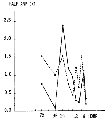
Fig. 12 Amplitudes of each fluctuating components, as obtained by harmonic analysis of cloud top T_{bb} . Solid line corresponds to the period before the beginning of rapid development and broken line corresponds to the period after the beginning of development.
