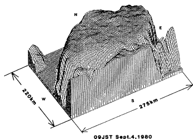
Fig. 5 Same as Fig. 4, except for 09JST Sept. 4, 1980 (Any dips can not be seen on the top of the cloud cluster.)
