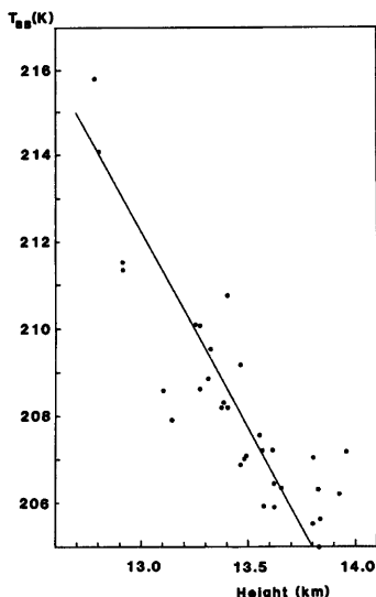
Fig. 10 The relation between radar-observed cloud top height and cloud top T_{BB} (adapted from Adler et al. 8) )
