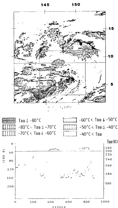
Fig. 2 (a) T_{BB} areal distribution for 09JST Sept. 4, 1980. Thresholds of T_{BB} are -80^\circ\text{C} , -70^\circ\text{C} , -60^\circ\text{C} , -50^\circ\text{C} and -40^\circ\text{C} .
