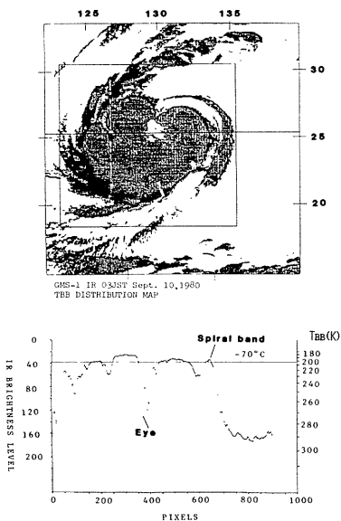
Fig. 7 (a) Same as Fig. 2 (a), except for 03JST Sept. 10, 1980
