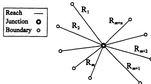
Figure 1. Schematic sketch of the star graph \Omega .
