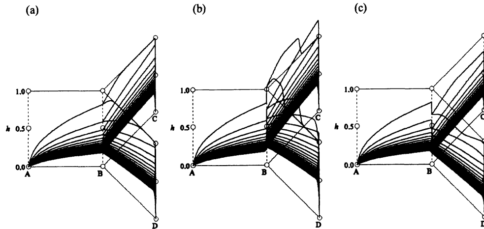
Figure 2. Computational results of the test problems.
