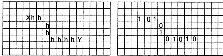
Figure 2: An edge giving the negation of the previous figure
