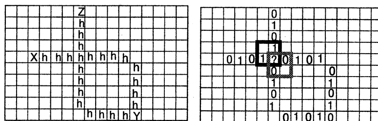
Figure 4: A gadget for a not-all-equal-3SAT clause.
