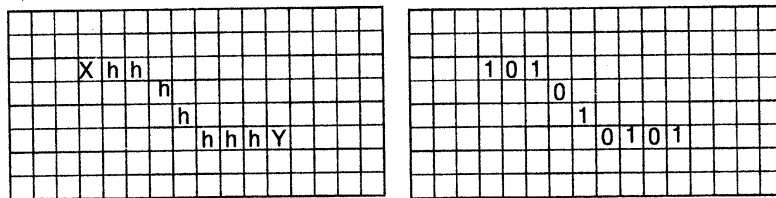
Figure 1: A gadget for an edge and its possible assignment.
