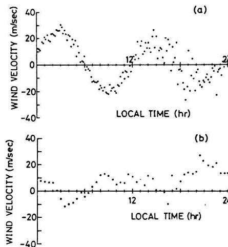
Fig. 5.4 Radial wind velocity versus local time. (a): artificially produced (averaged in every 10 minutes). (b): observed during 21-25 April, 1978 (averaged in every 30 minutes).
