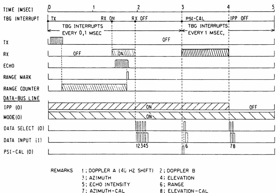
Fig. 3.21 A pulse scheme of measurement during one transmission in mode 2 controlled by IOC. Inter pulse period is variable, but is representatively set equal to 5 msec.
