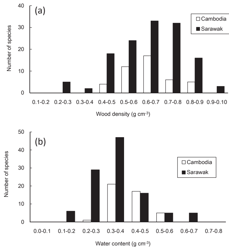
Fig. 1 Histograms of wood density (a) and water content (b) in Cambodia and Sarawak.
