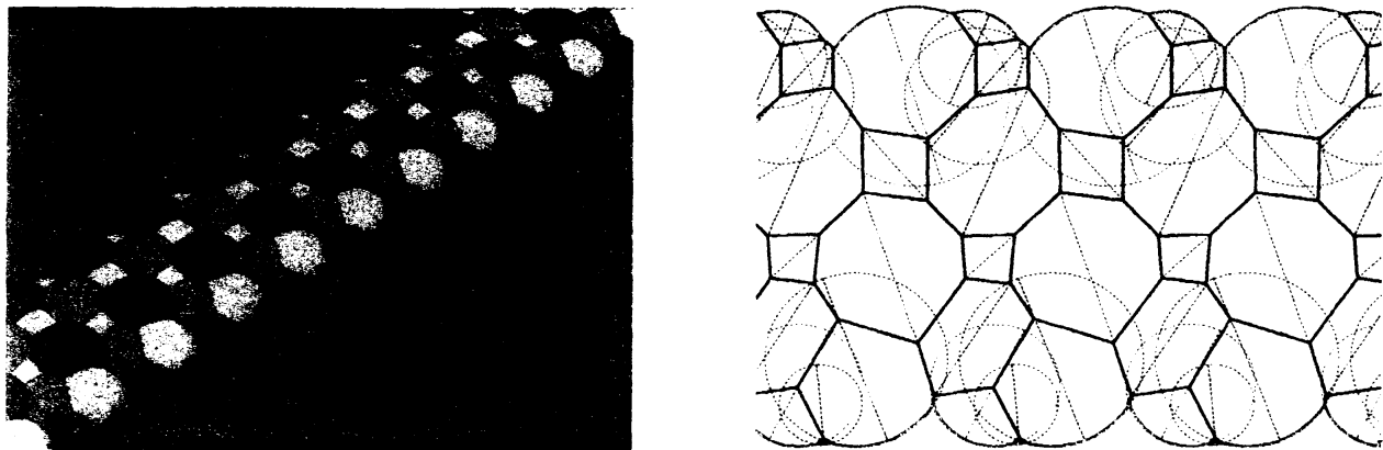
Figure 1: Ford domain of a generic quasifuchsian punctured torus group
