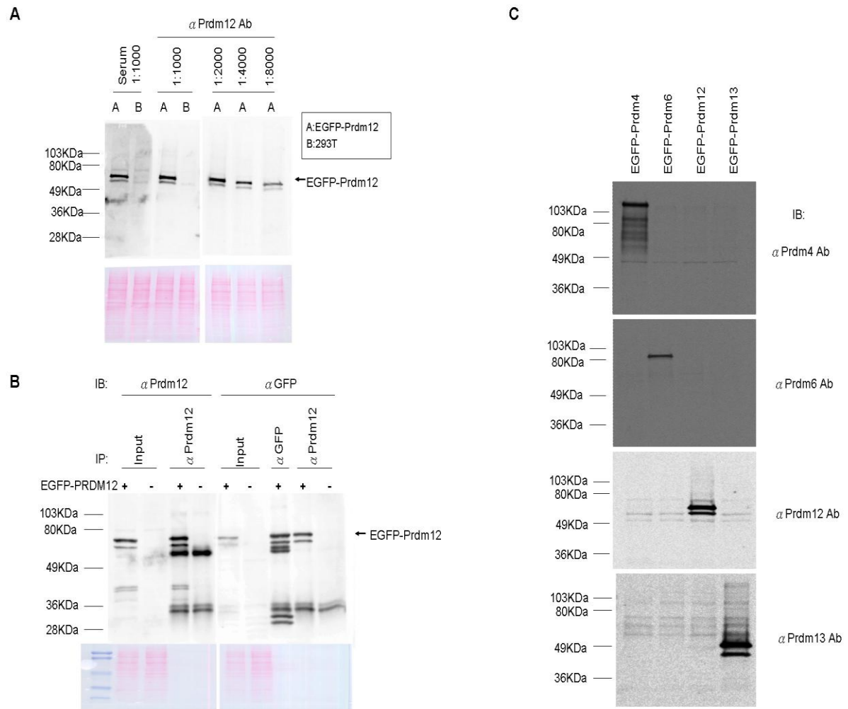
Fig. 2-7: (A) Anti-Prdm12 antibodies were serially diluted to detect EGFP-Prdm12 by western blot analysis. A: cell lysates contained over-expressed EGFP-Prdm12. B: HEK293T cell lysates were used as negative control. Original serum was used as a positive control. (B) Anti-Prdm12 antibodies could be used for immunoprecipitation. Anti-GFP antibody was used as a positive control. The EGFP-Prdm12 proteins isolated by anti-Prdm12 antibody were also confirmed by anti-GFP antibodies. (C) EGFP-Prdm4, EGFP-Prdm6, EGFP-Prdm12 or EGFP-Prdm13
