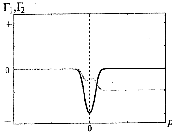
Figure 11: The profiles of the heterogeneous perturbations for jump type. Here black line is for \Gamma_1 , and gray line is for \Gamma_2 . This figure is obtained by numerical computation of the Gray-Scott model.
