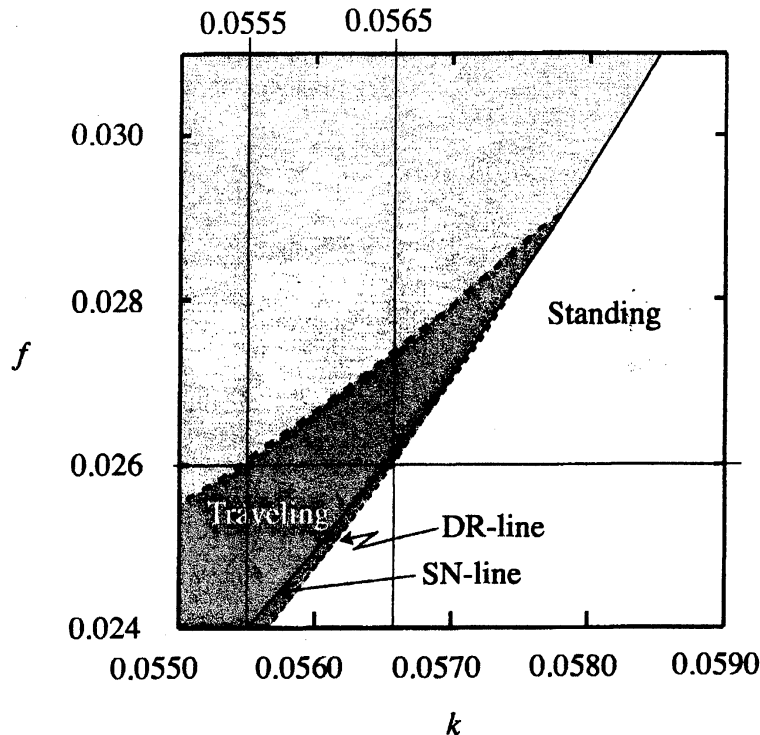
Figure 4: (k, f) -phase diagram. Here DR-line is the drift-bifurcation line, and SN-line is the saddle-node bifurcation line. The boundary between the splitting domain and the traveling domain is a Hopf bifurcation line. The cross point between DR-line and SN-line is the codim 2 point.
