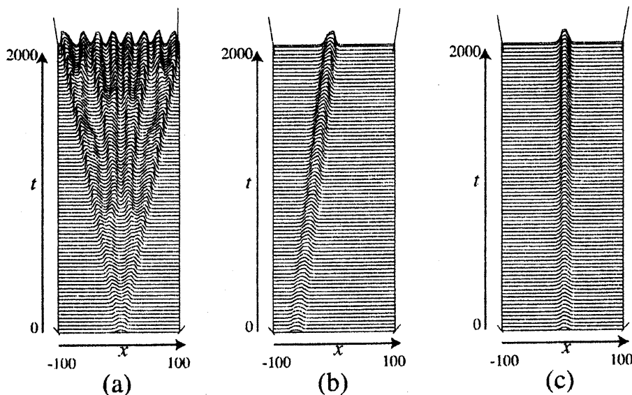
Figure 3: Dynamics of system (1) observed with numeric calculations for f = 0.026 , \epsilon = 0 , \Delta t = 0.05 and \Delta x = 0.25 . (a) Splitting pulse ( k = 0.0550 ), (b) Traveling pulse ( k = 0.0560 ) and (c) Standing pulse ( k = 0.0570 )
