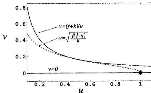
Figure 2: The nullclines of (1) for \epsilon = 0 intersect at only one point (u, v) = (1, 0) ; v = (f+k)/u and v = \sqrt{f(1-u)/u} do not intersect.
