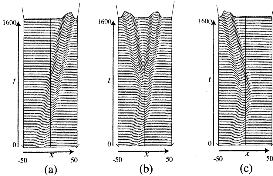
Figure 7: Heterogeneity causes a variety of pulse dynamics. (a) Penetration ( f = 0.026, k = 0.0557, \epsilon = 2.0 \times 10^{-4} ), (b) Splitting ( f = 0.026, k = 0.0557, \epsilon = 7.0 \times 10^{-4} ), (c) Rebound ( f = 0.026, k = 0.0557, \epsilon = 1.2 \times 10^{-3} ). The coefficient k(x) for the Gray-Scott model (1) has a heterogeneity of jump type as in Fig. 1, which exists at the center of the interval. The integrations are carried out with \Delta t = 0.05 , -50 \leq x < 50 and \Delta x = 0.125 .
