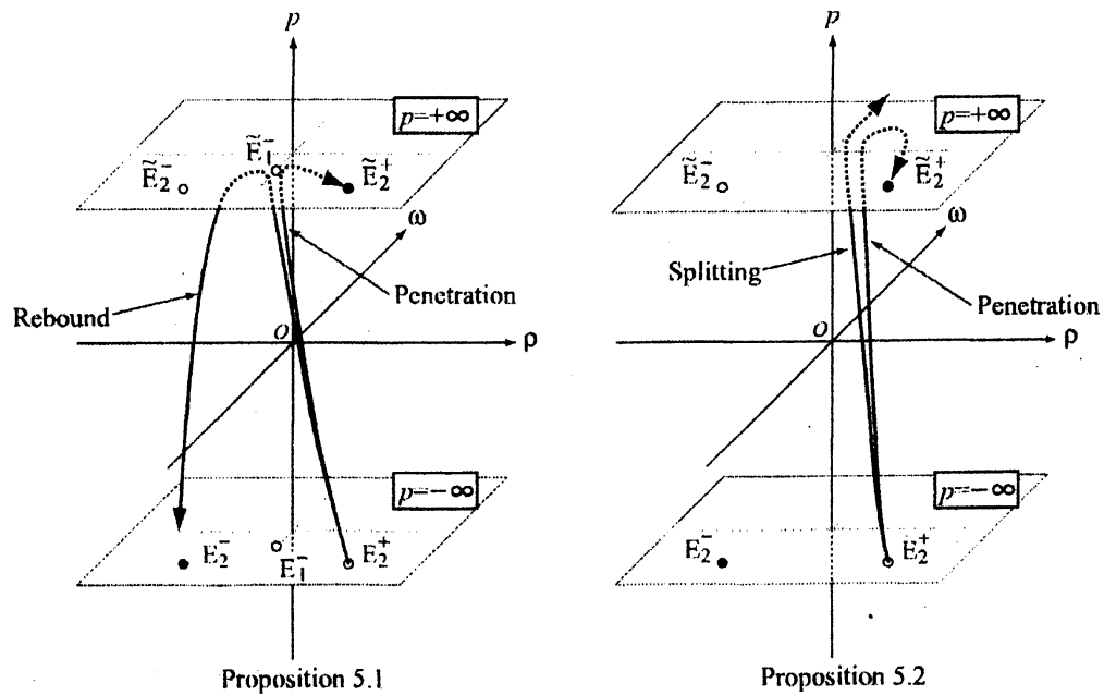
Figure 13: Schematic phase portrait for (8). Black and white circles indicate stable and unstable stationary solutions respectively.
