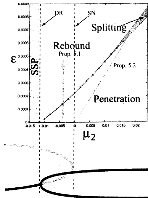
Figure 12: Phase diagram for (8) with parameter values corresponding to the Gray-Scott model. Here \mu_1 = -0.1 , s = -1 , \theta_1 = 0.93 , \theta_2 = 0.11 , C_2 = 0.85 . SSP stands for stable standing pulse, DR means drift bifurcation, and SN presents saddle-node bifurcation.
