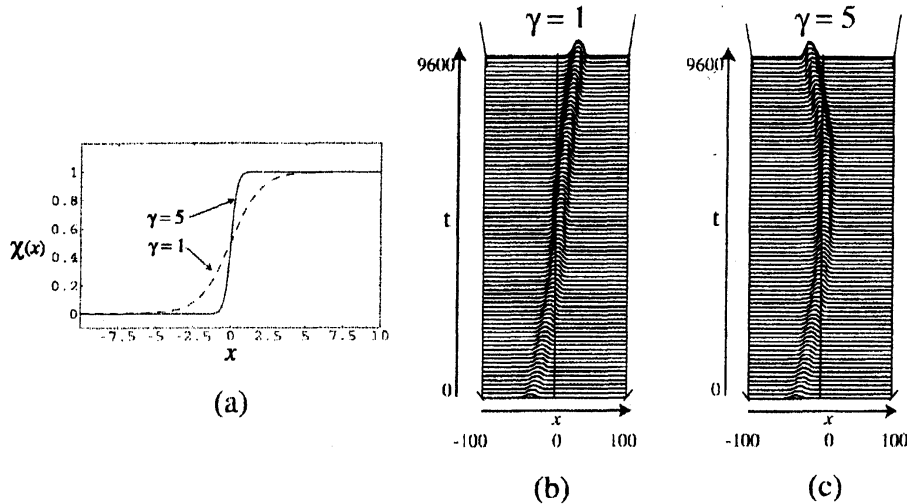
Figure 14: When the slope of heterogeneity becomes less steep, the pulse can penetrate. The profile of \chi(x) is illustrated by (a). For f = 0.026, k = 0.05652, \epsilon = 3.2 \times 10^{-5} , the pulse penetrate when \gamma = 1 (see (b)), however it turns back when \gamma = 5 (see (c)).
