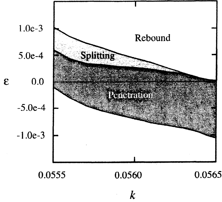
Figure 8: Response of the pulse in heterogeneous media for the Gray-Scott model with k(x) given by (1) with respect to k and \epsilon .
