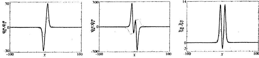
Figure 9: The profiles of the associated adjoint eigenfunctions at the codim 2 point for the Gray-Scott model. The black and gray line are for v -component and u -component respectively.
