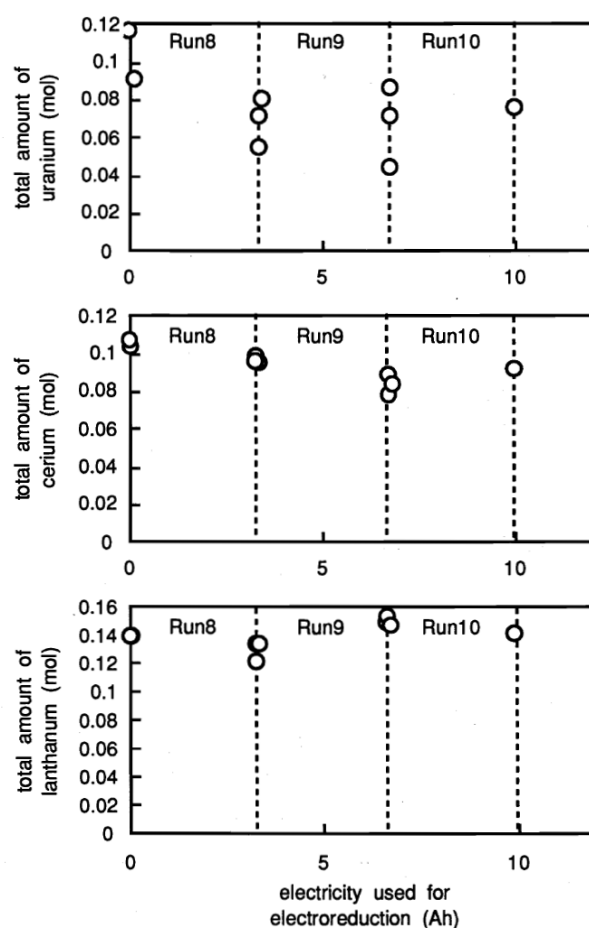
Fig. 3-10 Mass balance of uranium, cerium and lanthanum in electrochemical reduction tests (anodic current density = 0.195 \text{ A/cm}^2 )
