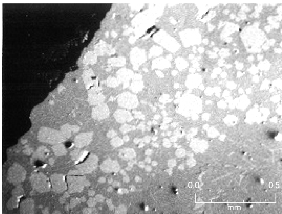
Fig. 4-11 SEM image of the LCC ingot shown in Fig. 4-7 (near the bottom)
