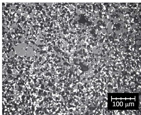
Fig. 7-16 Metallograph of the central region of the reduction product from Ca-1
