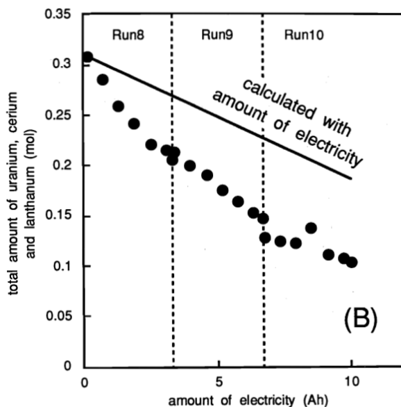
Fig. 3-11 Total amount of uranium, cerium and lanthanum in salt in electrochemical reduction tests : (A) anodic current density = 0.293 A/cm 2 , (B) 0.195 A/cm 2
