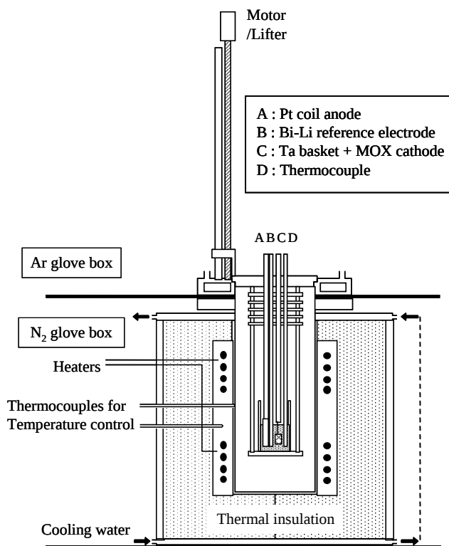
Fig. 7-2 Schematic view of the experimental apparatus
