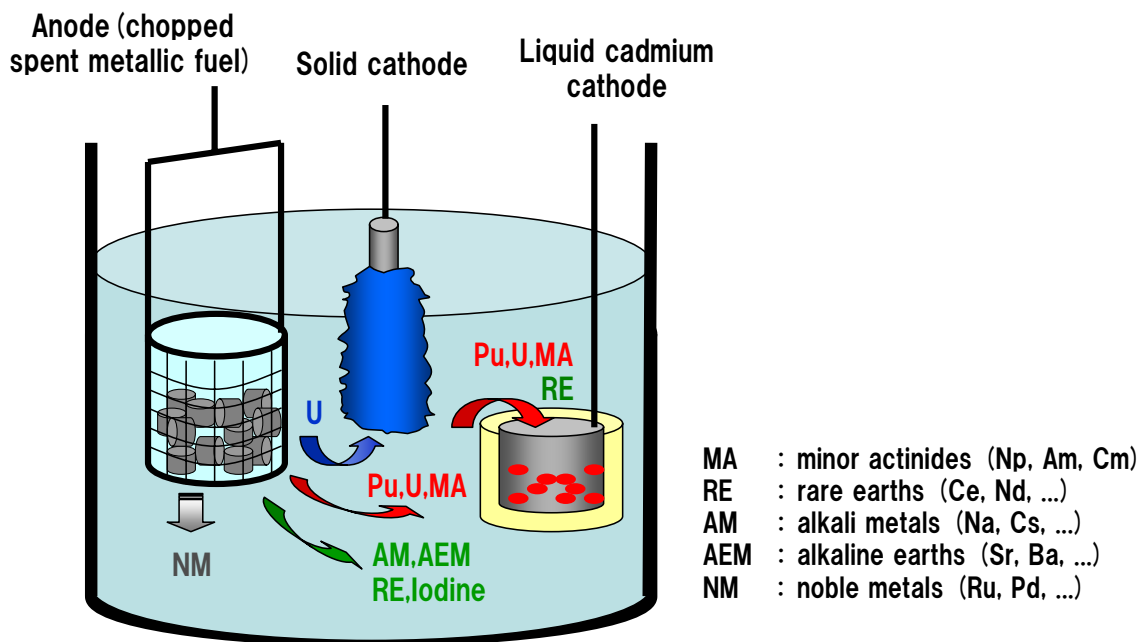
Fig. 5-1 Schematic diagram of electrorefining step for spent metallic fuel
