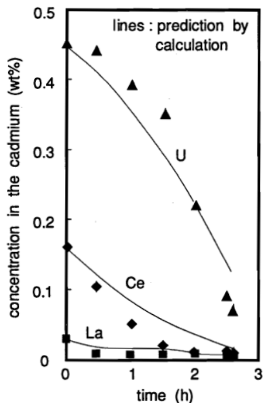
Fig. 3-5 Change of composition of liquid cadmium layer in electrotransport tests
