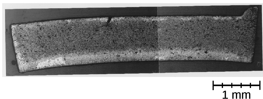
Fig. 7-11 Total section view of the reduction product from Li-2
