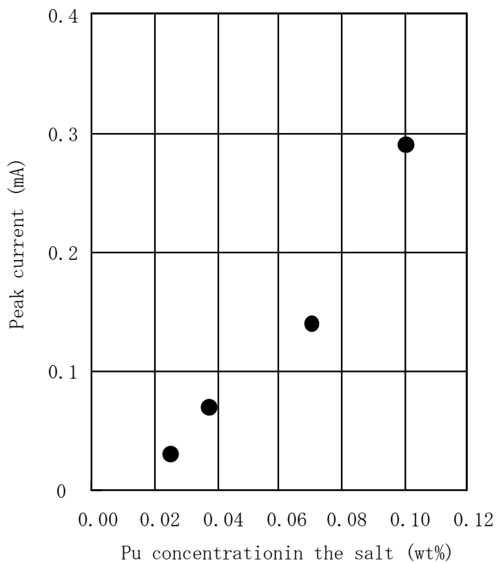
Fig. 6-8 Concentration dependence of peak height in SWV curves for LiCl-KCl-PuCl 3 (at lower Pu concentration)
