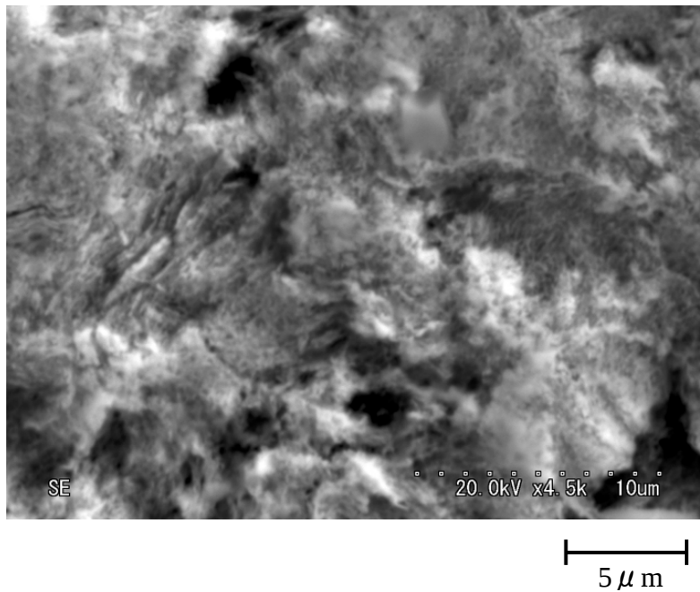
Fig. 5-3 Microstructure of remaining zirconium in anode residue [2]
