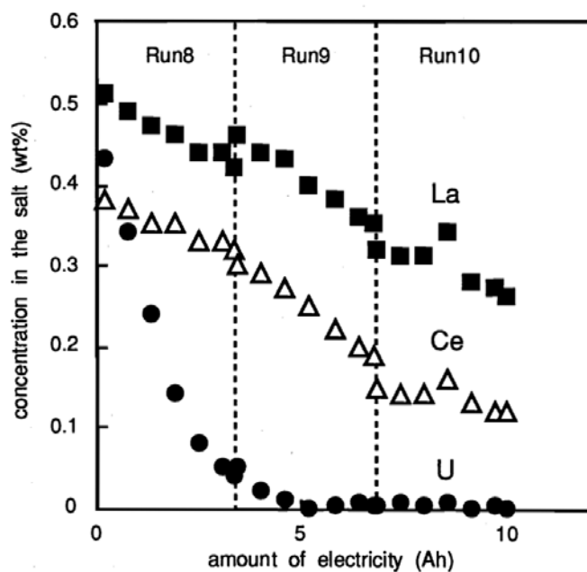
Fig. 3-9 Change of composition of molten salt electrolyte in electrochemical reduction tests (anodic current density = 0.195 \text{ A/cm}^2 )
