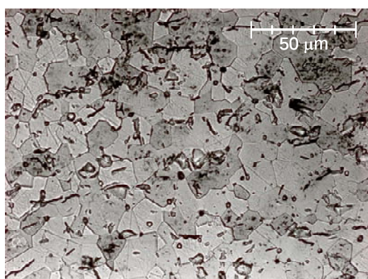
Fig. 7-3 Ceramograph of MOX-a pellet (Pu/(U+Pu) = 9.45 wt %) before electrochemical reduction
