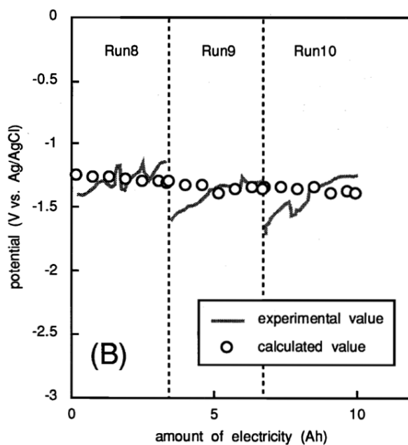
Fig. 3-12 Change of anode potential in electrochemical reduction tests : (A) anodic current density = 0.293 A/cm 2 , (B) 0.195 A/cm 2
