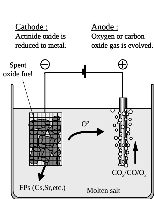
Fig. 7-1 Schematic diagram of the electrochemical reduction process
