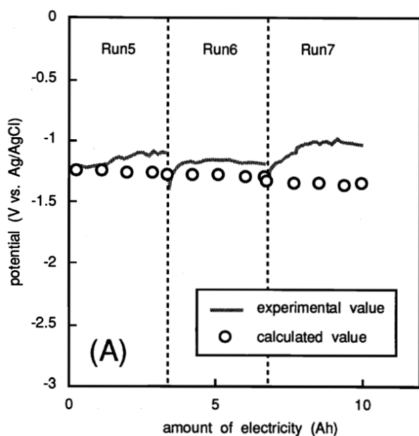
Fig. 3-12 Change of anode potential in electrochemical reduction tests : (A) anodic current density = 0.293 A/cm 2 , (B) 0.195 A/cm 2
