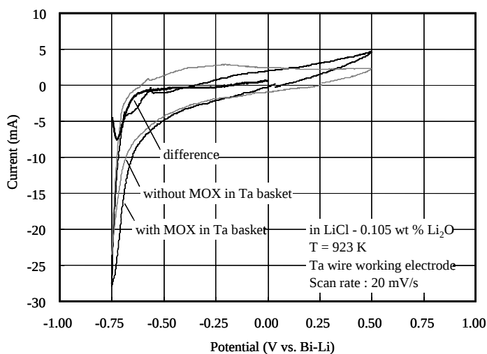
Fig. 7-4 Cyclic voltammograms measured in LiCl electrolyte with/without MOX in cathode
