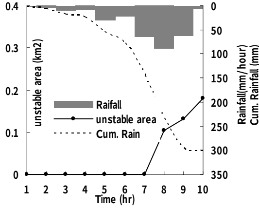
Fig. 5 Rainfall Event on 1973/10/26 and calculated unstable area
