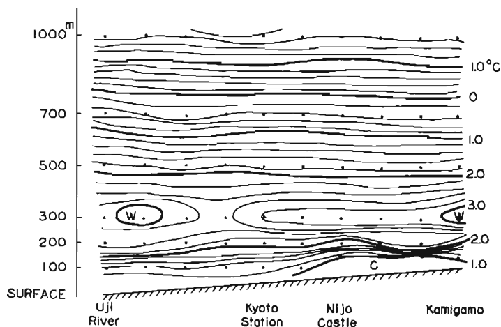
Fig. 4 N-S vertical temperature cross section in the Kyoto basin, observed from 6:48 to 7:42 Mar. 14, 1967.
