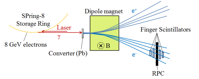
Figure 4: The experimental setup of the beam test. The beam test was performed at the LEPS beamline. High energy gamma rays hit a Pb converter. The electrons from the converter were bent by the dipole magnet and irradiated to RPCs. The triggered area was defined by four finger scintillators to be 1 \times 2 \text{ cm}^2 .
