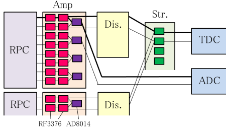
Figure 3: The schematic drawing of the FEE system.
