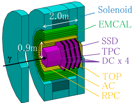
Figure 1: The LEPS2 spectrometer with the solenoid magnet moved from BNL. A SSD, a TPC and four DCs are used for the charged-particle tracking. The energy of photons is measured by EMCAL. The PID is done by TOPs, ACs and RPCs.
