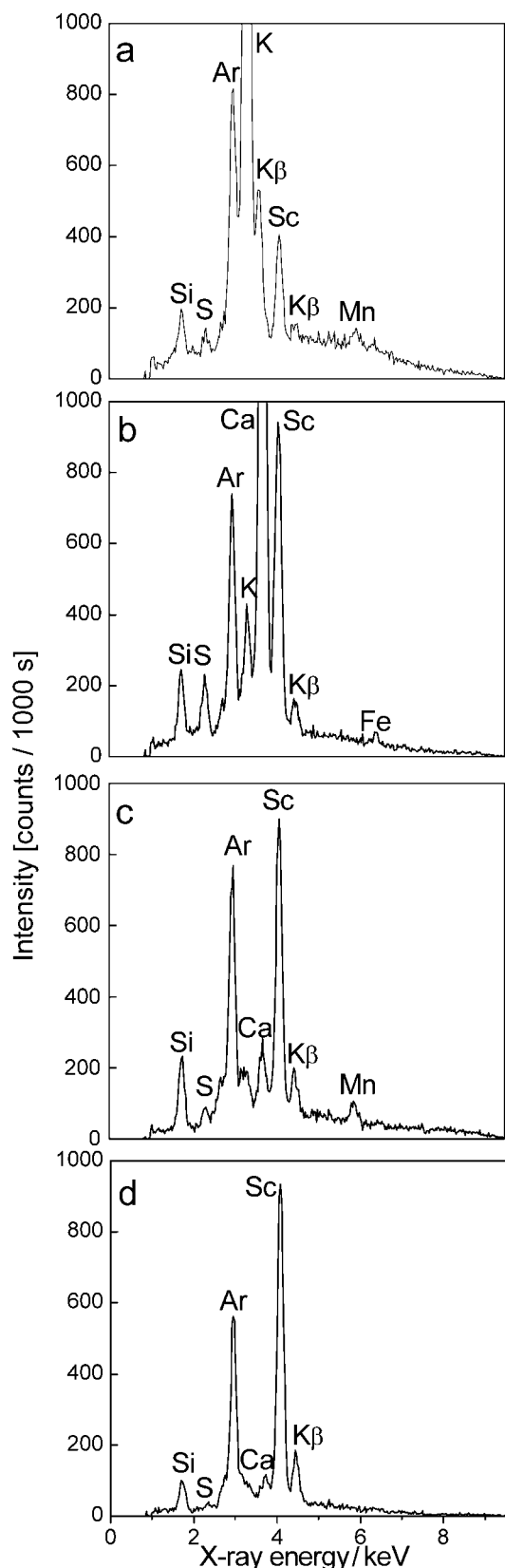
Fig. 2 Representative measured total reflection X-ray fluorescence spectra of dry residues of (a) oolong tea, (b) water in a pool, (c) a leaching solution of a plastic toy, and (d) distilled water boiled in a glass beaker
