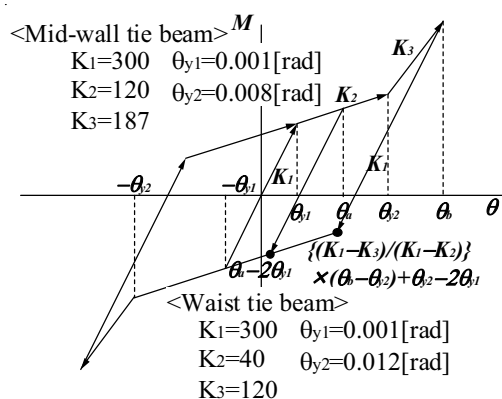
Fig. 30 Hysteresis model of moment-rotation relationship at the joint of column-mid wall tie beam and waist tie beam
