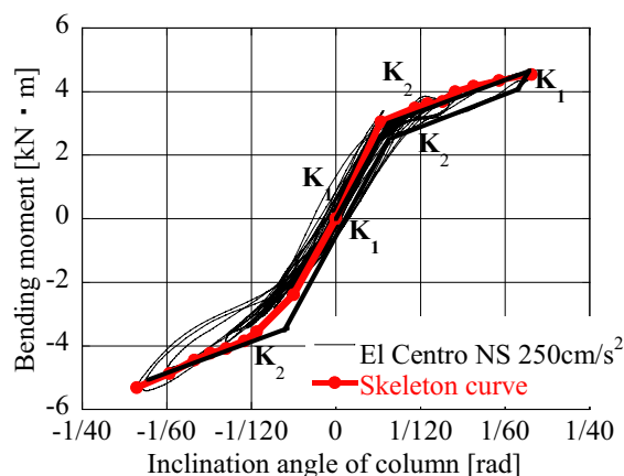
Fig. 31 Average of moment-rotation relationship at all the bottom of column of basic specimen in X-direction under El Centro NS
