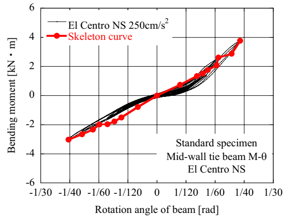
Fig. 12 Moment-rotation relationship at the joint of column-mid wall tie beam of basic specimen in X-direction under El Centro NS
