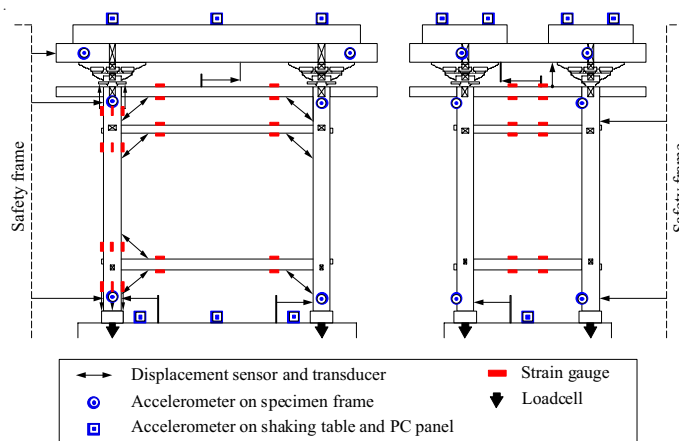
Fig. 6 Allocation of instruments and sensors
