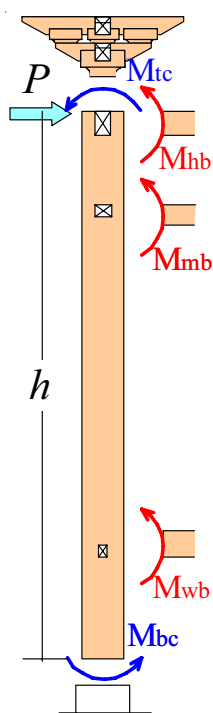
Fig. 18 Moment equilibrium of column
