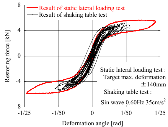
Fig. 10 Comparison between hysteretic restoring force under shaking table test and static lateral loading test (simple frame specimen)
