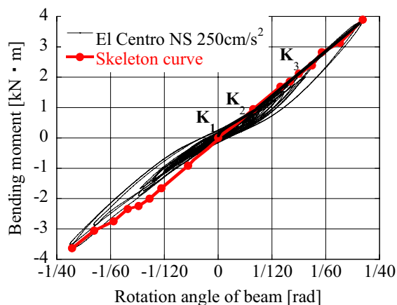
Fig. 27 Average of moment-rotation relationship at all the joint of column-mid wall tie beam of basic specimen in X-direction under El Centro NS
