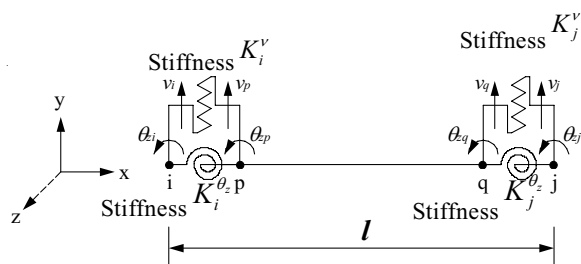
Fig. 25 Element model of beam with rotational spring and shear spring
