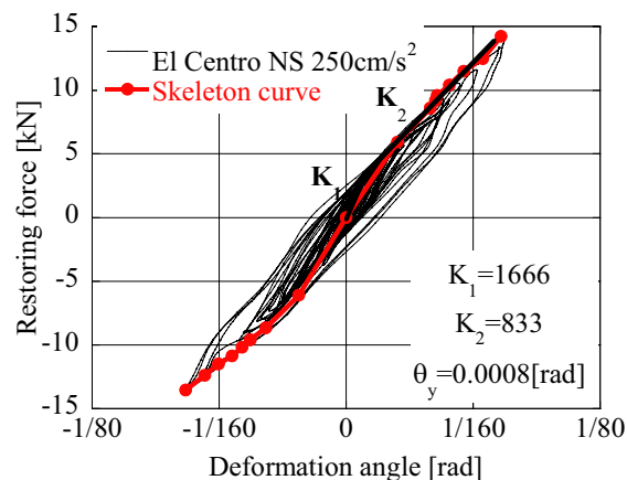
Fig. 33 Restoring force of bracket complex in X-direction under El Centro NS
