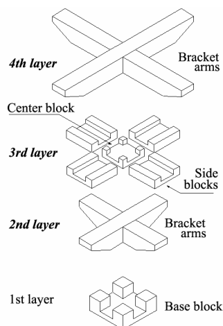
Fig. 3 Details of bracket complex
