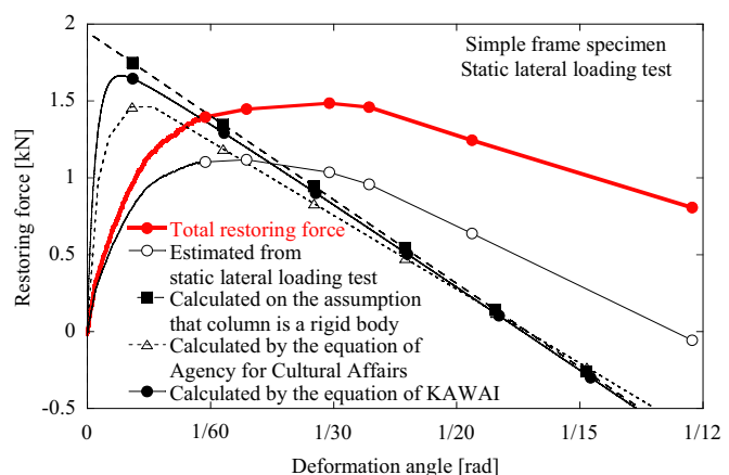
Fig. 24 Skeleton curves of total restoring force and restoring force due to column rocking on the static test of simple frame specimen
