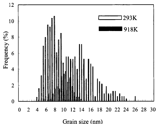
FIG. 4. Grain size dispersion of the \text{Co}_3\text{O}_4 thin films formed at T_s of 293 and 918 K.
