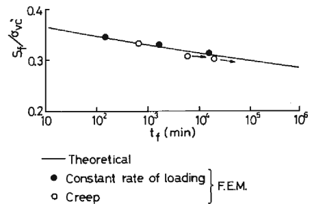
Fig. 9 Shear strengths plotted against durations of loading.
