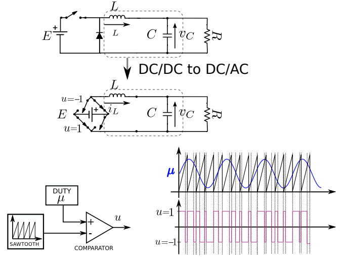
FIG. 2: Working of the buck-type inverter.
