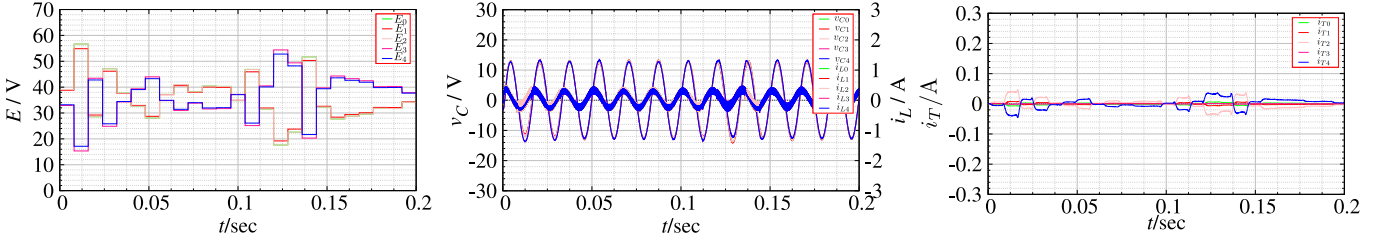
FIG. 7: Behaviour of unbalanced AC-grid with varying input voltages under PBC.
