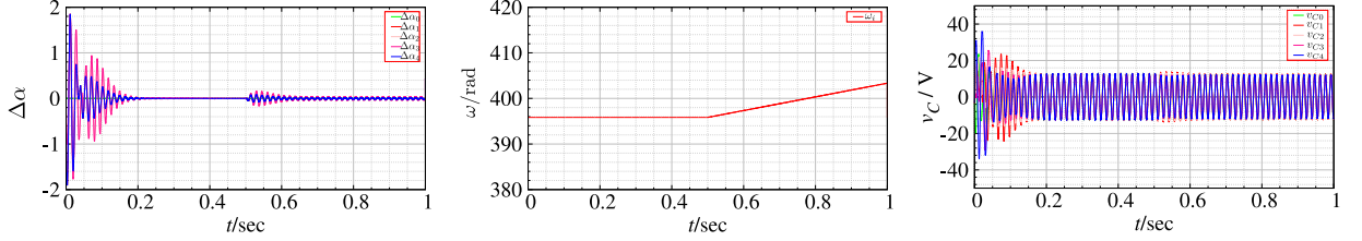
FIG. 11: Linear change in the frequency of the sinusoidal PWM reference.
