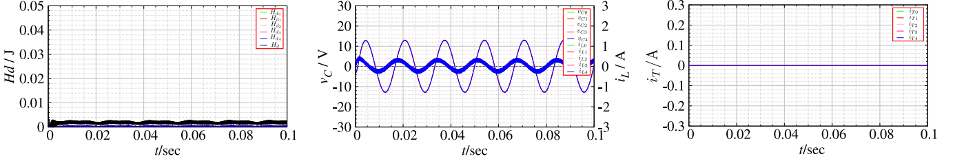
FIG. 6: Time evolution of AC grid with PBC. Here, \bar{v}_{Cn} is set with parameters A_n = 13 , f_n = 60 Hz.
