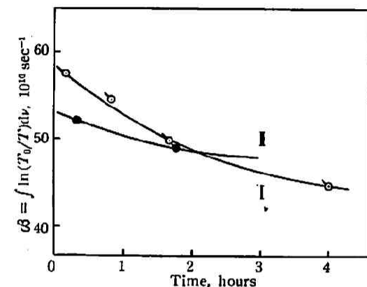
Fig. 2 The values of \alpha\beta against the time after the end of filling at total pressures of 1 \text{ kg/cm}^2 (curve I) and 24 \text{ kg/cm}^2 (curve II) for Le of \text{CS}_2 = 0.0144 cm at N. T. P.
