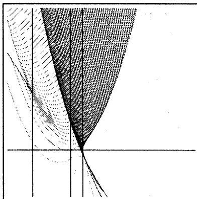
Figure 8: Moduli space with parabolic curves: -10 \leq \sigma_1 \leq 20 , -10 \leq \sigma_2 \leq 30 . The right white region is the degree +2 region, and the wedged white region in the left is the degree -2 region.
