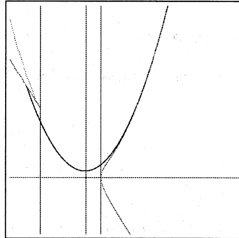
Figure 7: Parabolic curve in the moduli space. In the case of a = -0.2 , -10 \leq \sigma_1 \leq 30 , -10 \leq \sigma_2 \leq 40
