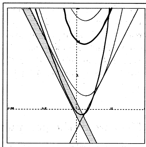
Figure 5: algebraic curve of degree 4 in the "classified" moduli space. Thick curve corresponds with r = 0.58 , thin curve corresponds with r = 0.7 .
