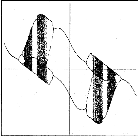
Figure 6: Period-doubling and period-halving bifurcation, -1.0 \leq r \leq 1.0 , -6.0 \leq x \leq 6.0 , a = -0.20
