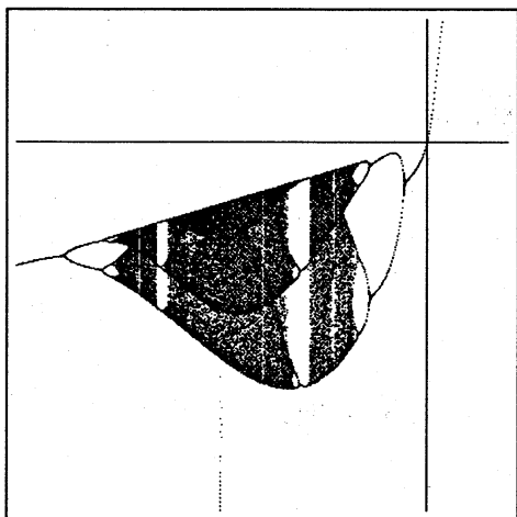
Figure 2: Non-monotone bifurcation, -25.0 \leq m \leq 5.0 , -3.0 \leq x \leq 1.0 , r = 0.54
