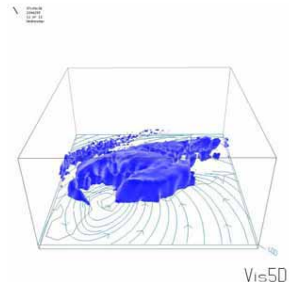
Fig.13 Bird eye view of simulation with MM5
