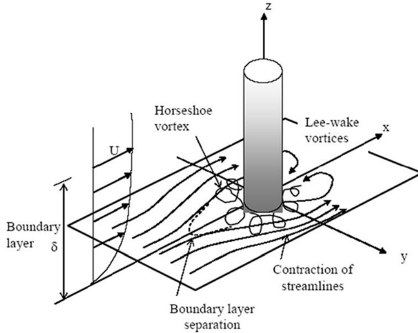
Figure 1-1. The change in the flow pattern and the boundary layer after being exposed to current (Sumer and Fredsøe 2002)
