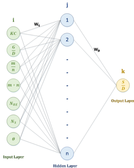
Figure 4-3. Scheme of the MLP network used in current study
