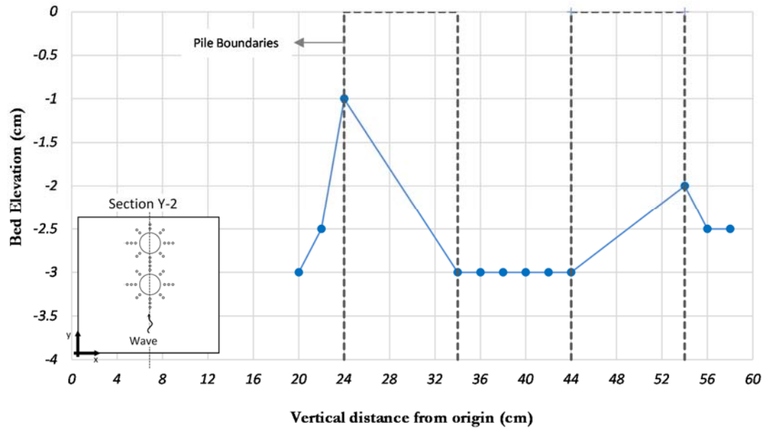
Figure 2-20. Bed profile of two piles along Y section for KC = 3.9
