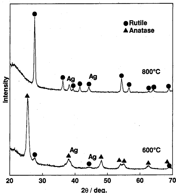
Fig. 5. XRD patterns of the coating films that were obtained by heating the gel films at 600 and 800°C measured using the thin-film attachment, Cu K\alpha radiation operated at 40 kV and 200 mA and a scanning rate of 2 deg./min.
