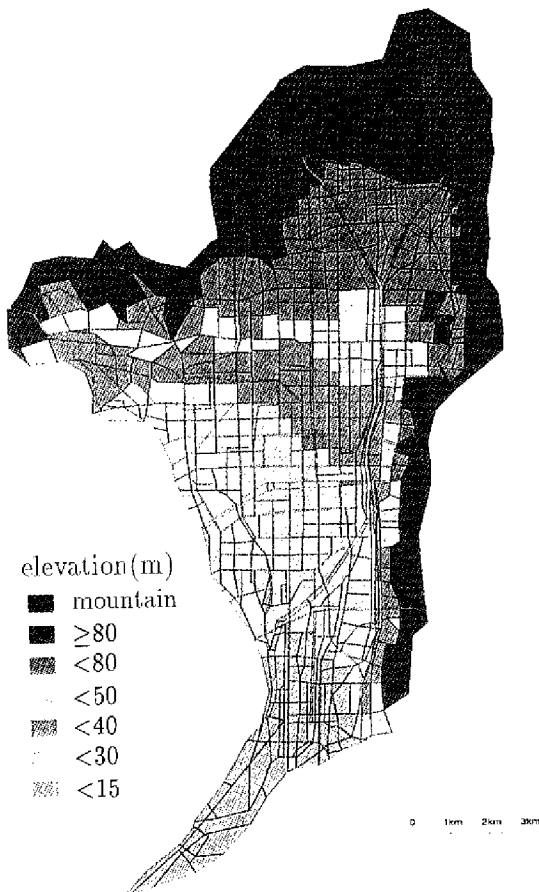
Fig.9 Ground elevation and network
