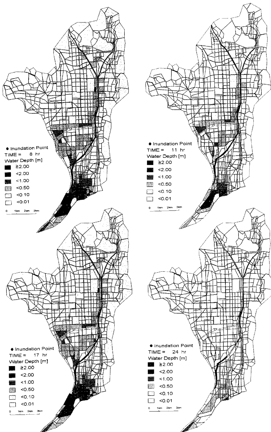
Fig.14 Temporal change of Inundation flow depth distribution
