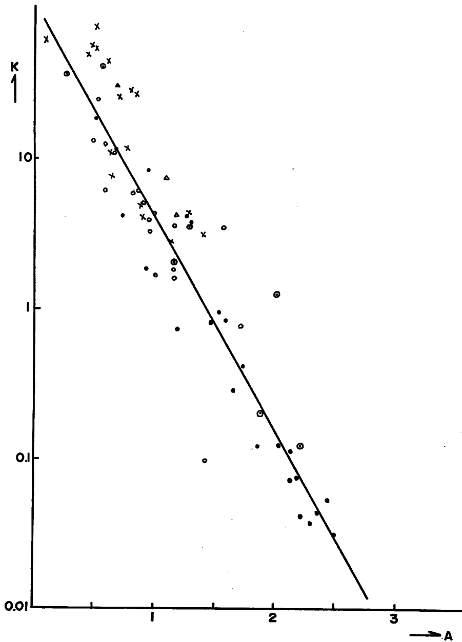
Fig. 2 The A-K relation showing the moved soil at the upper part of the critical displacement line.
