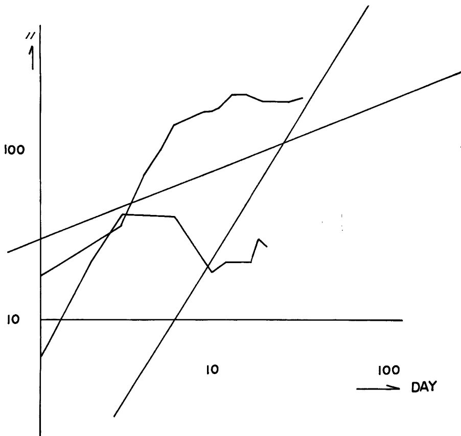
Fig. 4 The estimation figure whether the surface had moved or not by the data gotten from tiltmeters.
