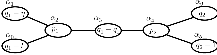
Figure 2. This figure denotes Dynkin diagram of type D_6^{(1)} .
