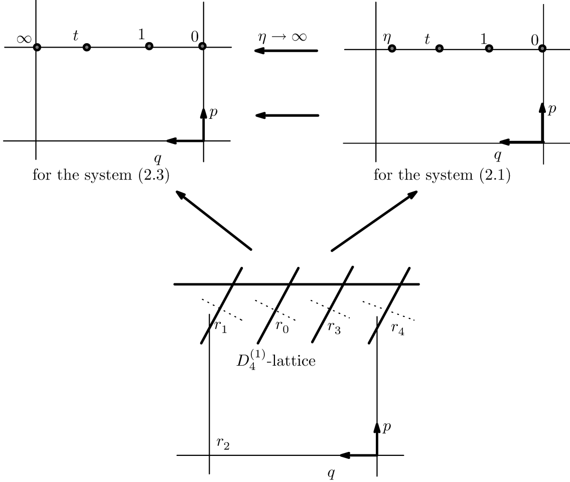
Figure 1. Each figure denotes the Hirzebruch surface. Each bullet denotes the accessible singular point of each system. It is well-known that each point can be resolved by blowing-up at two times (see [6], [8], [9]). By these transformations, we obtain the rational surface of type D_4^{(1)} for each system.
