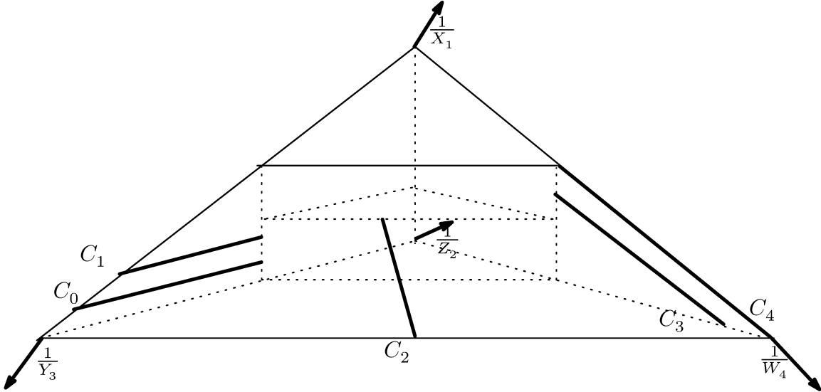
Figure 4. This figure denotes the boundary divisor \mathcal{H} of \mathcal{S} . This divisor is covered by eight affine spaces U_3 \cup U_4 \cup U_6 \cup U_7 \cup \cdots \cup U_{11} . The bold lines C_i ( i = 0, 1, \dots, 4 ) in \mathcal{H} denote the accessible singular loci of the system (1.1) (see Lemma 5.2).
