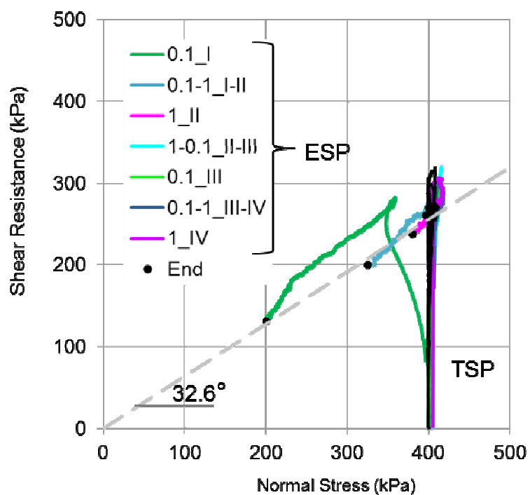
Fig. A.4.3 Stress path of all stages (I-VIII), TSP- total stress path, ESP- effective stress path.
