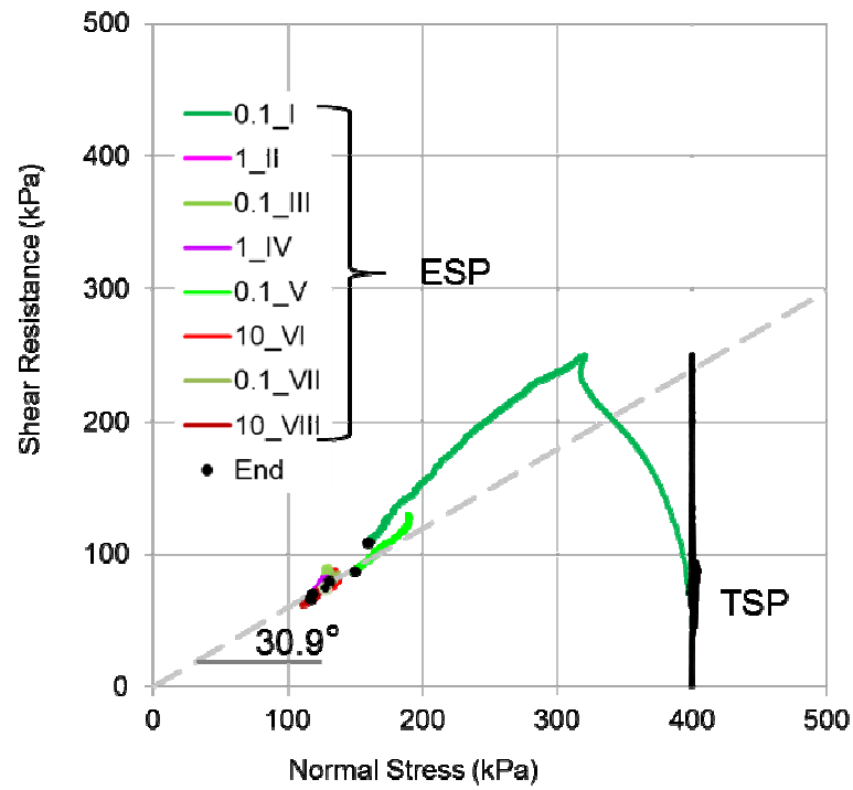
Fig. A.2.3 Stress path of all Stages (I-VIII), TSP- total stress path, ESP- effective stress path.
