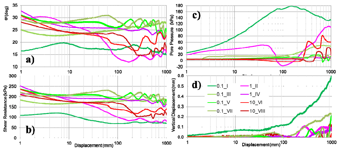
Fig. A.10.2 Shear displacement and a) Effective friction angle ( \Phi' ), b) Shear resistance, c) Pore pressure and d) Vertical displacement.
