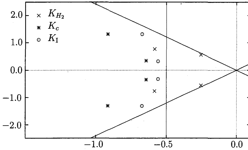
Figure 3.1: Pole locations under K_{H_2} , K_c and K_I
