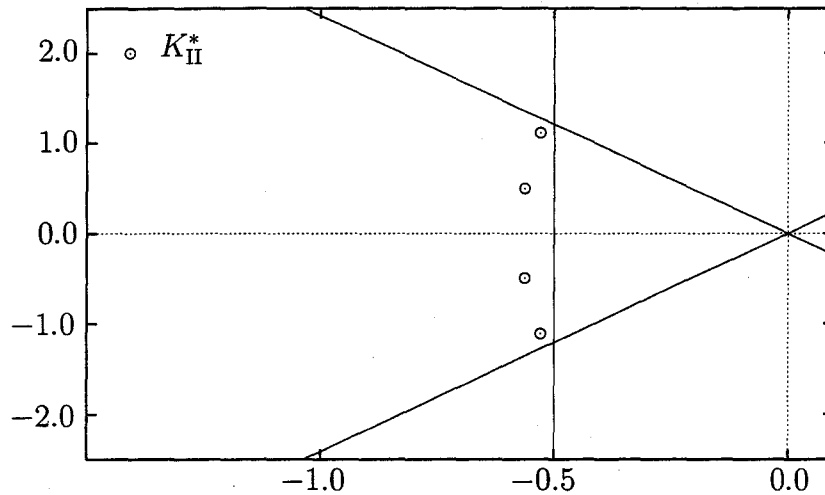
Figure 3.4: Pole locations under K_{\Pi}^*
